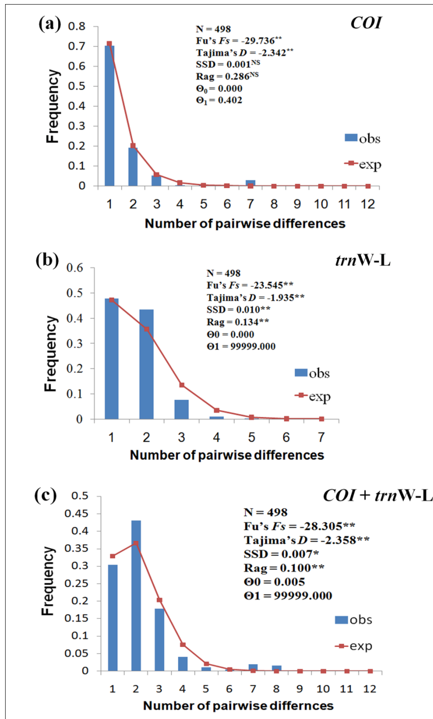
Figure S3 Pairwise mismatch distributions for Saccharina japonica inferred from mtDNA sequences. The abscissa indicates the number of pairwise differences between compared sequences. The ordinate is frequency for each value. Bar represent the observed distribution of pairwise frequencies, while the solid line shows the expected distribution.
