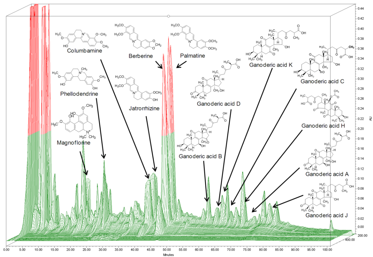
Supplemental Figure 1: HPLC fingerprint for FAHF-2 showing structure of compounds found in the major peaks.
