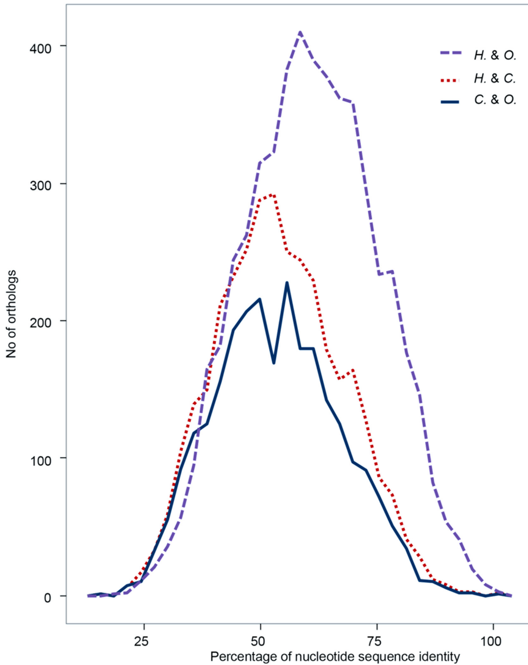
Figure S3 Distribution of the number of orthologs between two species per percentage of gene sequence identity. H. : Histoplasma capsulatum ; C. : Candida albicans ; O. : Ophiostoma novo-ulmi
