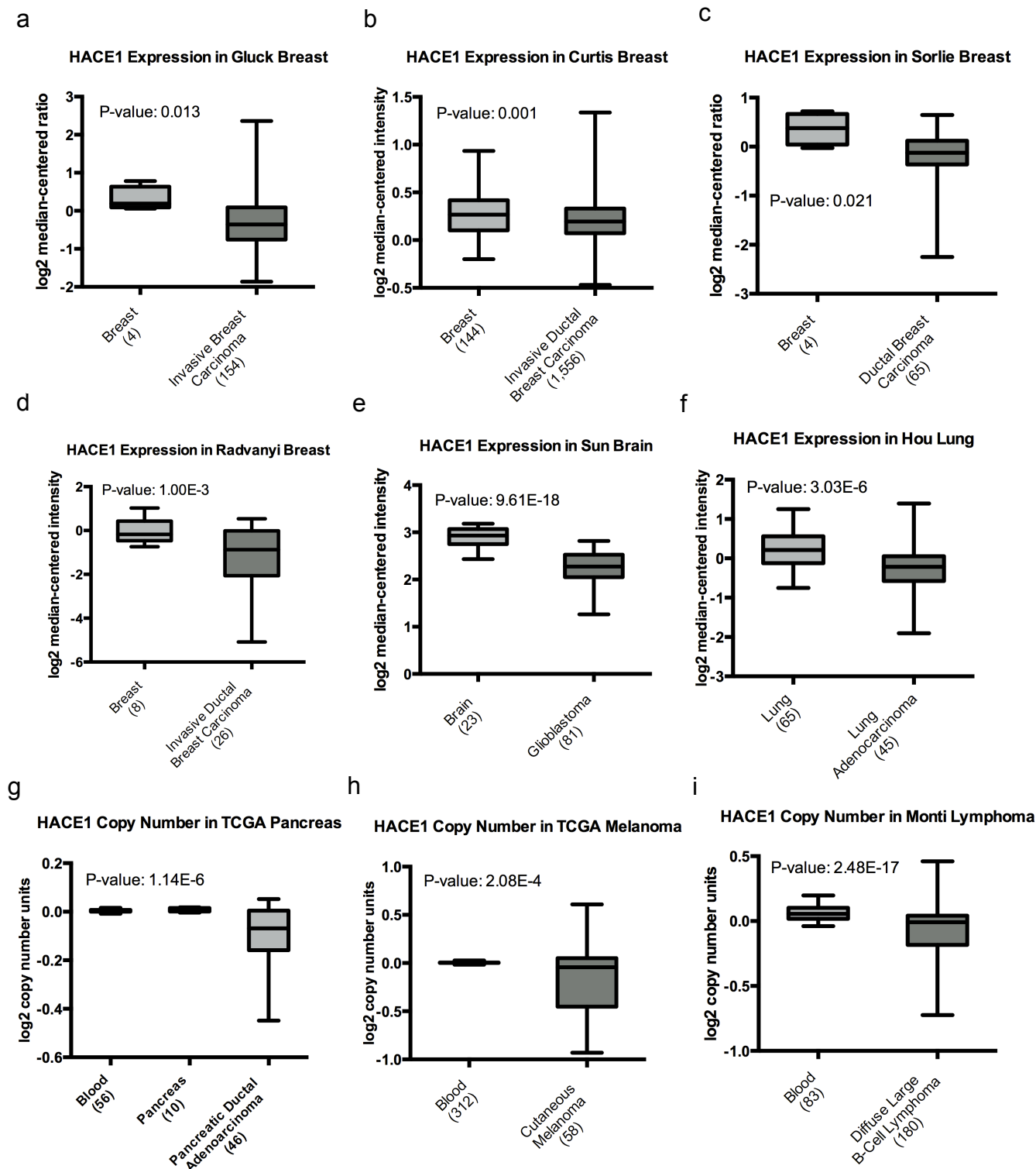
Supplementary Figure 1 – Reduced HACE1 expression in multiple breast cancer datasets. HACE1 mRNA expression in normal breast and breast carcinoma in (a) Gluck Breast, (b) Curtis Breast, (c) Sorlie Breast, and (d) Radvanyi Breast clinical datasets. HACE1 mRNA expression in (E) normal brain and glioblastoma, (F) normal lung and lung adenocarcinoma. HACE1 DNA copy number in (G) blood, normal pancreas, and pancreatic ductal adenocarcinoma, (H) blood and cutaneous melanoma, and (I) blood and diffuse large B-Cell lymphoma. All figures are modified from OncoPrint™ (Compendia Bioscience, Ann Arbor, MI) was used for analysis and visualization. P-value determined by Student’s t-test.
