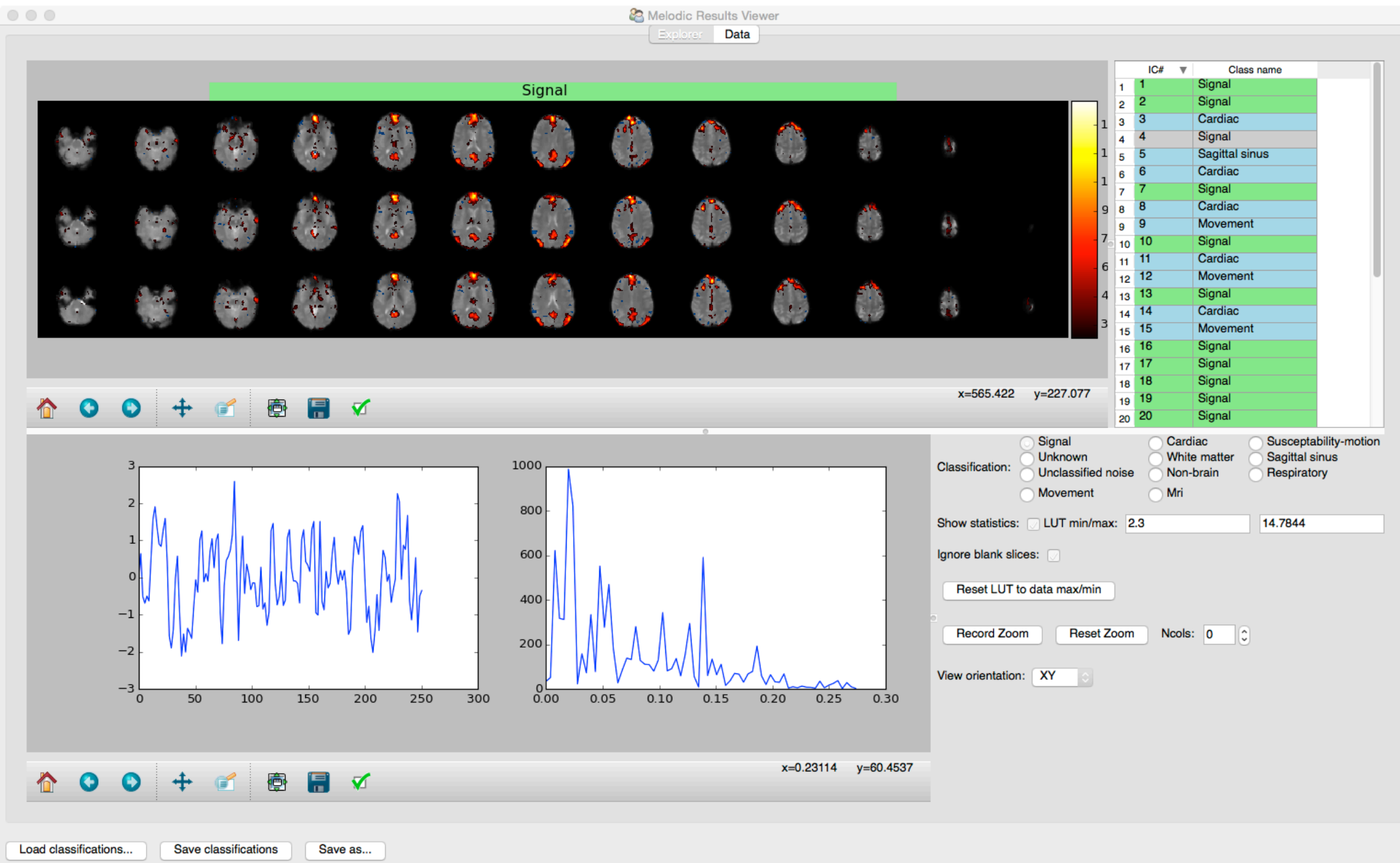
Fig. S1c. Signal ICA component (Default Mode Network)
