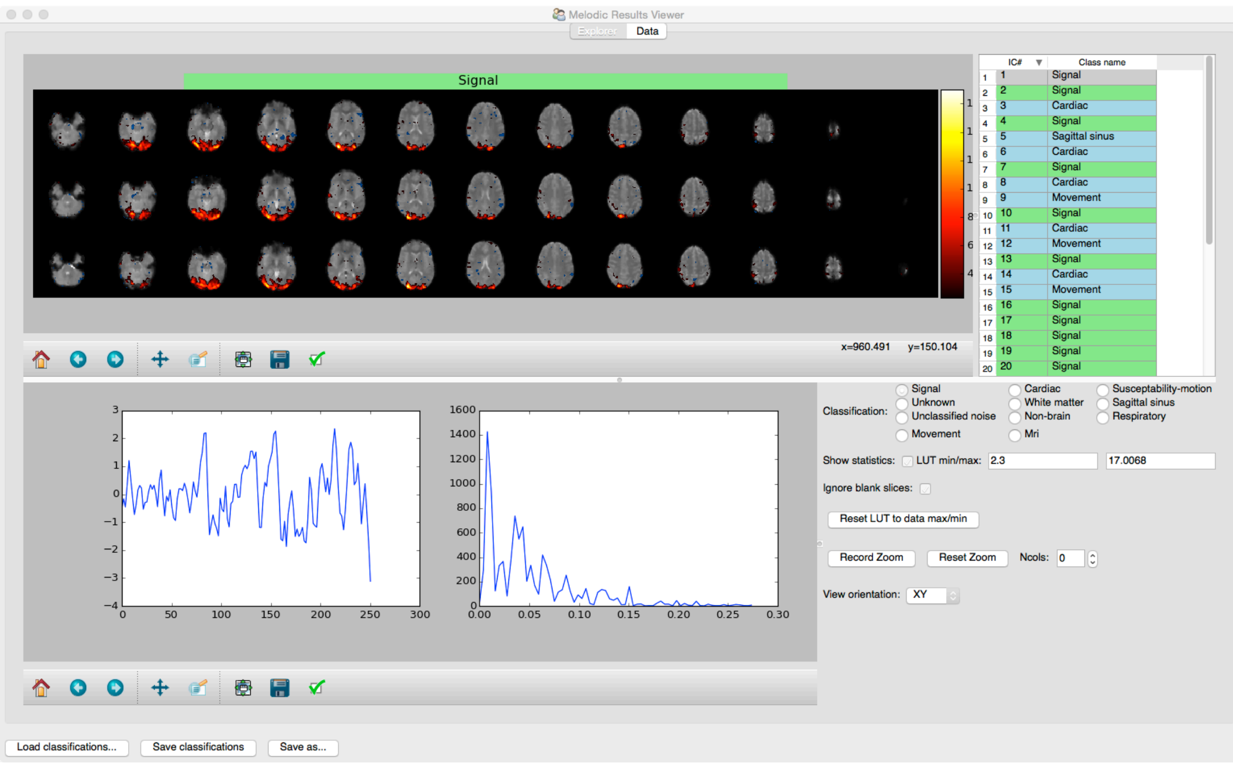
Fig. S1a. Signal ICA component (Occipital Visual)
