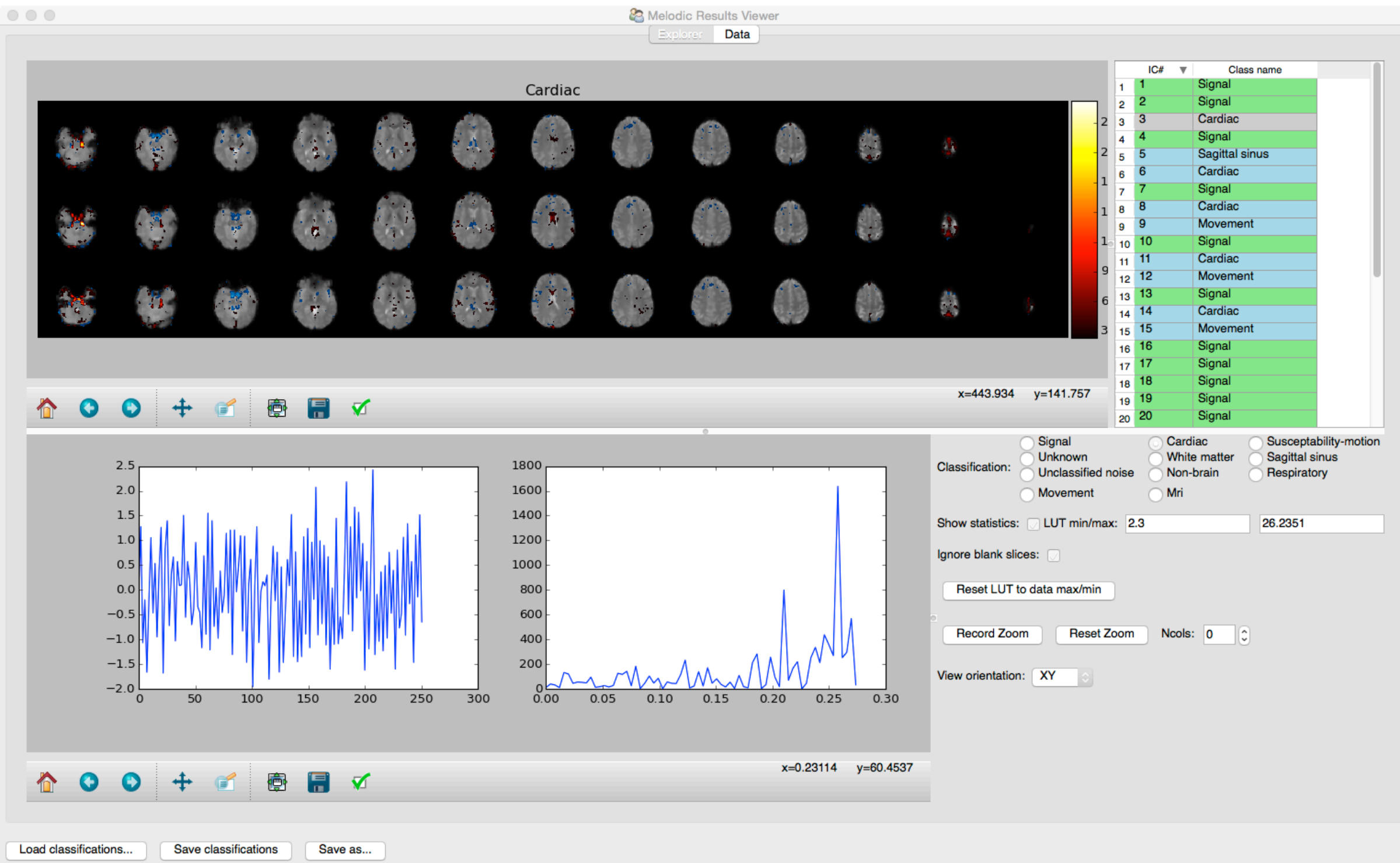
Fig. S1d. Artefactual ICA component (Cardiac)
