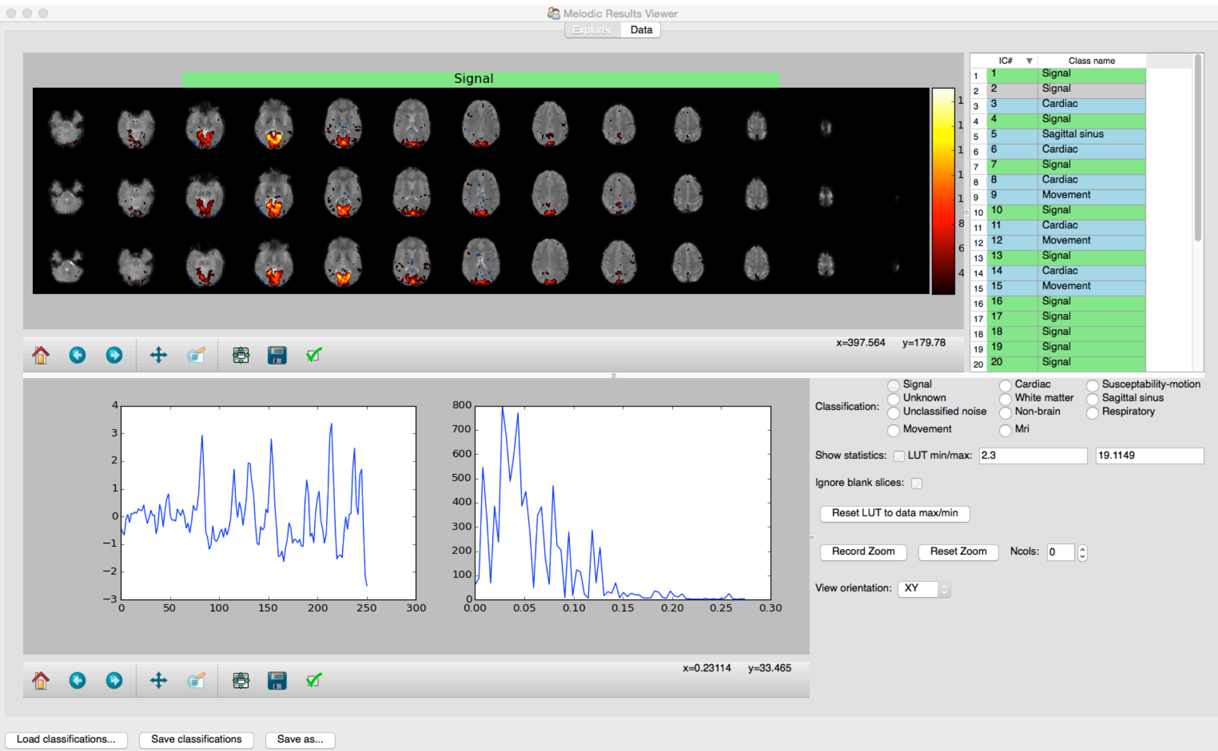
Fig. S1b. Signal ICA component (Medial Visual)
