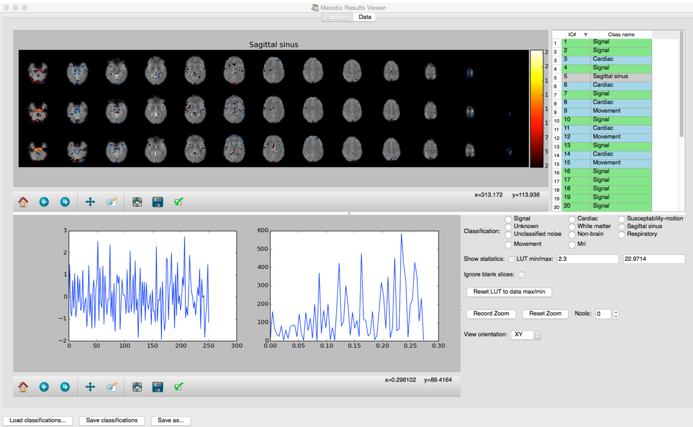
Fig. S1e. Artefactual ICA component (Veins)
