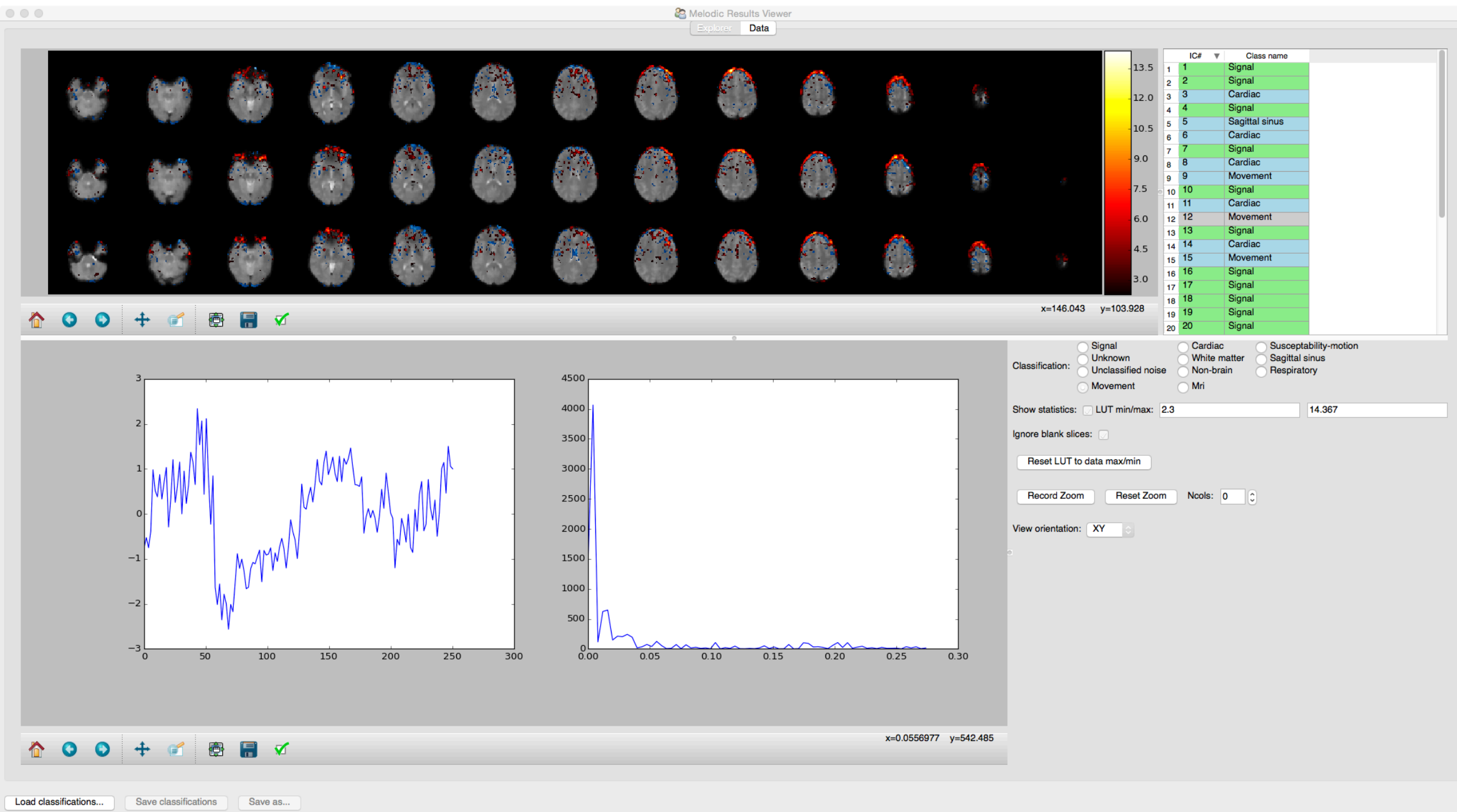
Fig. S1f. Artefactual ICA component (Movement)
