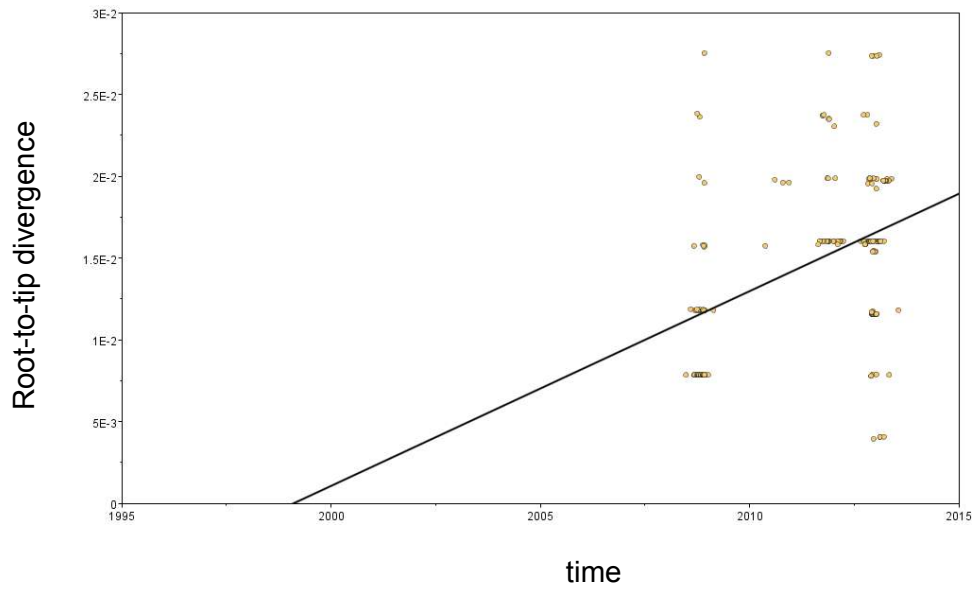
Figure S3. Root-to-tip linear regression of NA1 strains circulating from May 2008 – April 2012.
