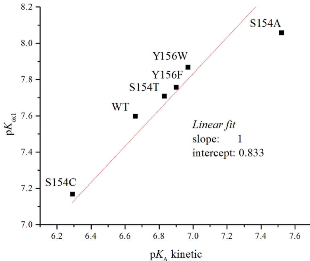
Figure S1: Correlation between pK_{ox1} and pK_A . Correlation between the pK_A value measured kinetically, which reflects the occupancy of the reaction complex, and the pK_{ox1} of H156, determined from the pH dependence of the redox potential in different mutant strains.
