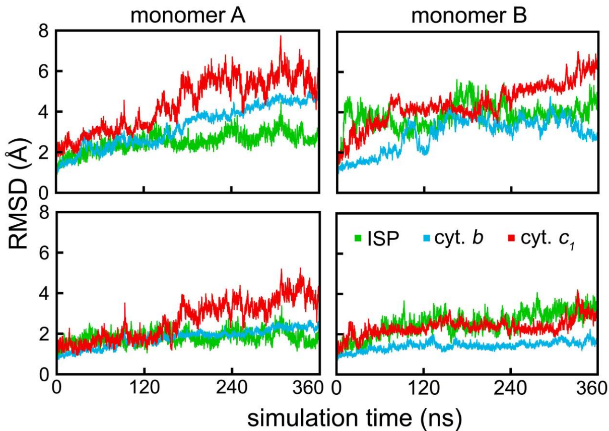
Figure S3: Equilibration of the bc_1 complex. RMSD values calculated for the protein subunits of the two monomers (A and B) of the bc_1 complex in case of Model I (Fig. 1). Upper panels: RMSD calculated for all atoms of the protein's backbone. Lower panels: RMSD computed only for the atoms of the secondary structure motifs that exclude bridges, coils and turns. All RMSD plots were computed with respect to the reference structure noted in Fig. S2.
