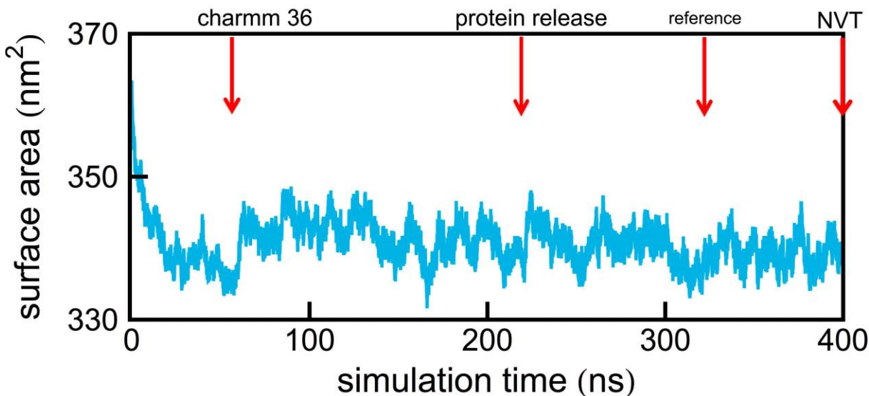
Figure S5: Lipid bilayer equilibration. Surface area of the lipid bilayer as a function of simulation time, calculated during the equilibration of Model II. The bc_1 complex proteins were released after 220 ns; up until this point the simulations of Model I and Model II were carried out identically. RMSD value calculations of the bc_1 complex protein subunits and the hydrogen bonding network analysis were performed with respect to the configuration of the system at 310 ns, as indicated by a vertical arrow marked “reference”. MD simulations beyond 400 ns were carried out in the NVT ensemble.
