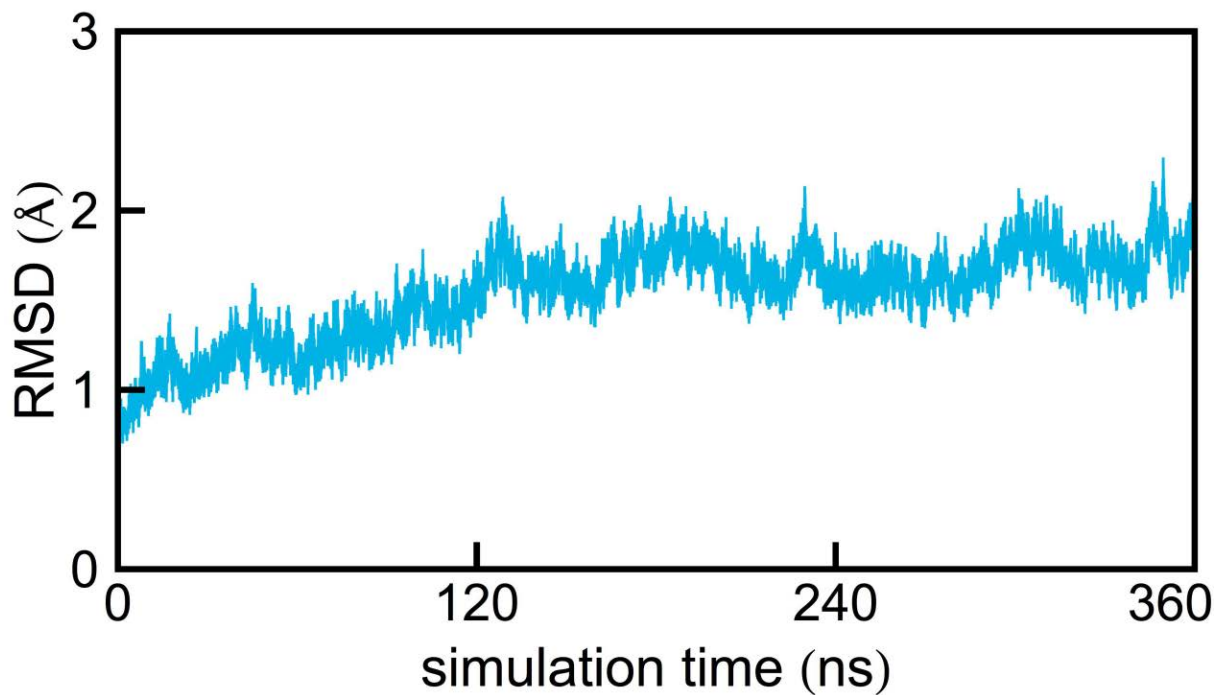
Figure S4: Equilibration of intermembrane helices. Shown are RMSD values calculated for the atoms of the transmembrane helices of the bc_1 complex in case of Model I. RMSD values were computed with respect to the reference structure noted in Fig. S2.
