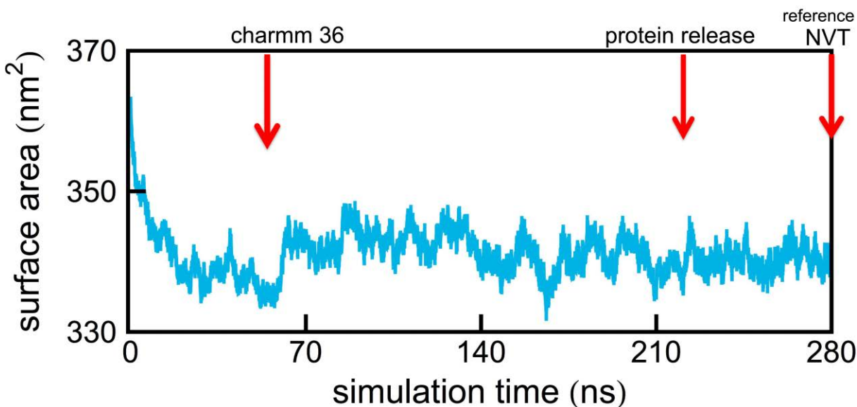
Figure S2: Lipid bilayer equilibration. Time evolution of the surface area of the lipid bilayer, calculated during the Model I equilibration. The first 60 ns were simulated with a combination of CHARMM 22 and 27 force fields, as done in, 13 while CHARMM 36 was used beyond 60 ns (point indicated with an arrow). The proteins of the bc 1 complex were constrained to the configuration of the crystal structure and subsequently released after 220 ns, as also indicated by a vertical arrow. MD simulations beyond 280 ns were continued in the NVT ensemble, and the configuration of the system at the 280 ns simulation instance was used as a reference structure in further analysis.
