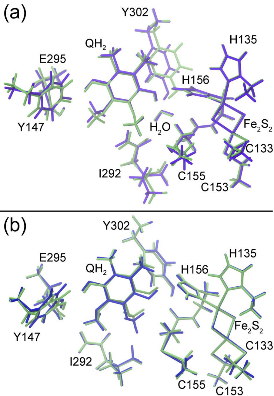
Figure S8: Comparison of quantum chemical optimizations of the Q o -site. Shown are aligned optimized structures of the Q o -site for Model I (a) and Model II (b) obtained using the B3LYP/6-311G(d) (lime) and B3LYP/6-311+G(d) (blue) methods. The structures were aligned to minimize the relative RMSD value which equals 0.37 Å and 0.33 Å in the case of Model I and Model II, respectively.
