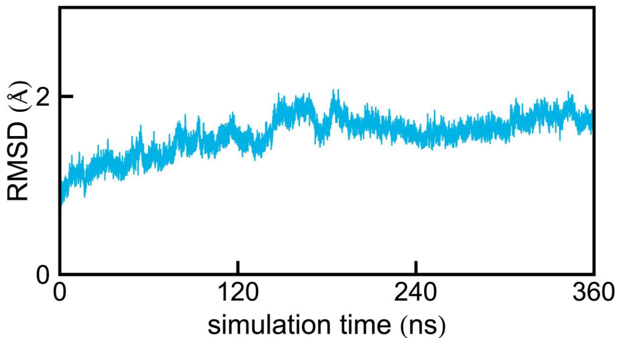
Figure S7: Equilibration of intermembrane helices. Shown are RMSD values calculated for the atoms of the transmembrane helices of the bc_1 complex in case of Model II. The RMSD values were computed with respect to the reference structure obtained after 310 ns of membrane and protein equilibration noted in Fig. S5.
