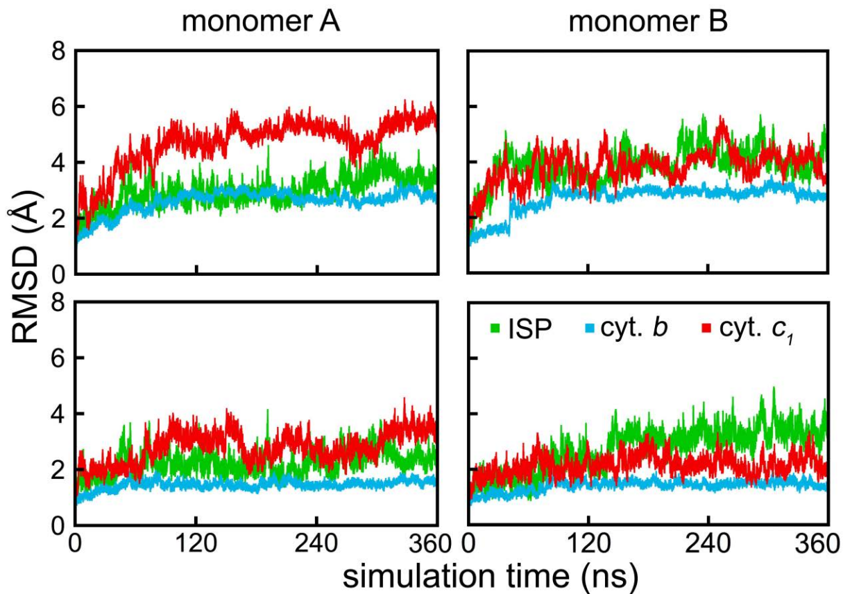
Figure S6: Equilibration of bc_1 complex. RMSD values calculated for the protein subunits of the two monomers (A and B) of the bc_1 complex in case of Model II (Fig. 1). Upper panels: RMSD calculated for all atoms of the protein's backbone. Lower panels: RMSD computed only for the atoms of the secondary structure motifs that exclude bridges, coils and turns. All RMSD plots are computed with respect to the reference structure noted in Fig. S5.
