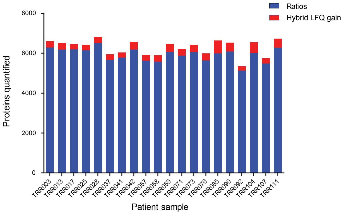
FIG. S1. Quantified proteomes of DLBCL patients employing the hybrid LFQ algorithm. Red bars indicate the gain from using the hybrid LFQ compared to using SILAC ratios alone.
