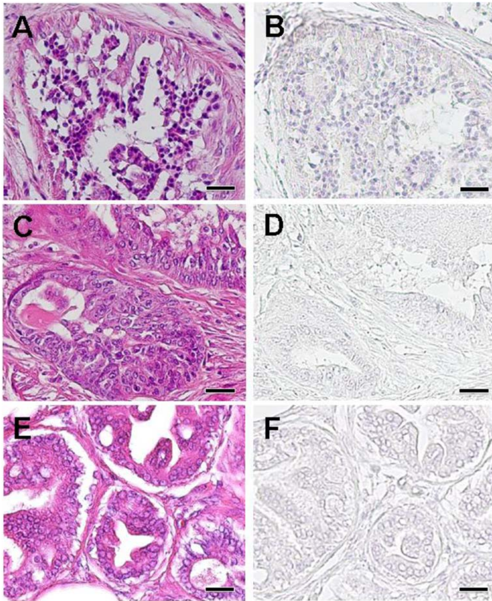
Supplemental Fig. 1. Histological and immunohistochemical images of the malignant tumor samples used for Western blotting.
