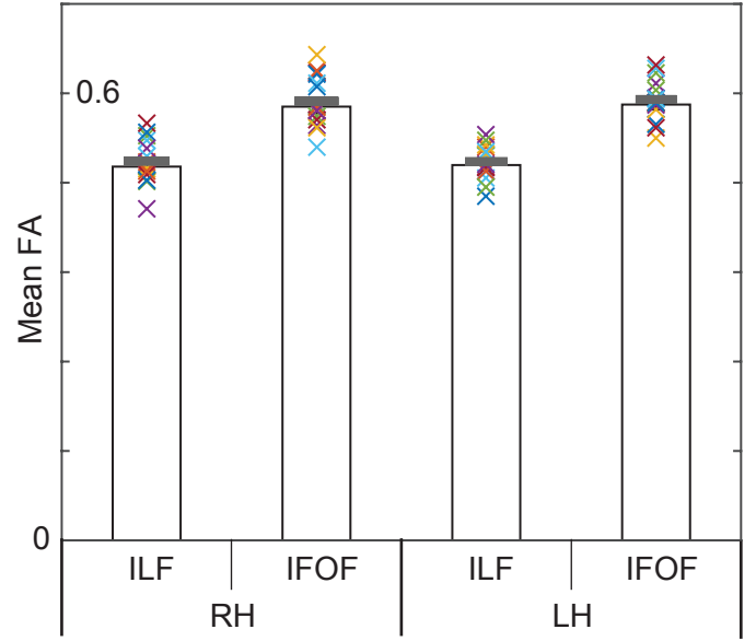
b. Fractional anisotropy in masked ILF and IFOF
