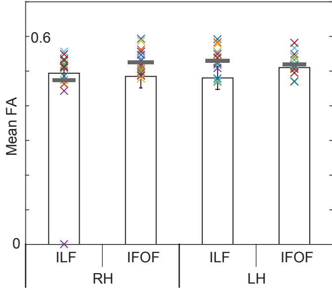
a. Fractional anisotropy in masked ILF and IFOF
