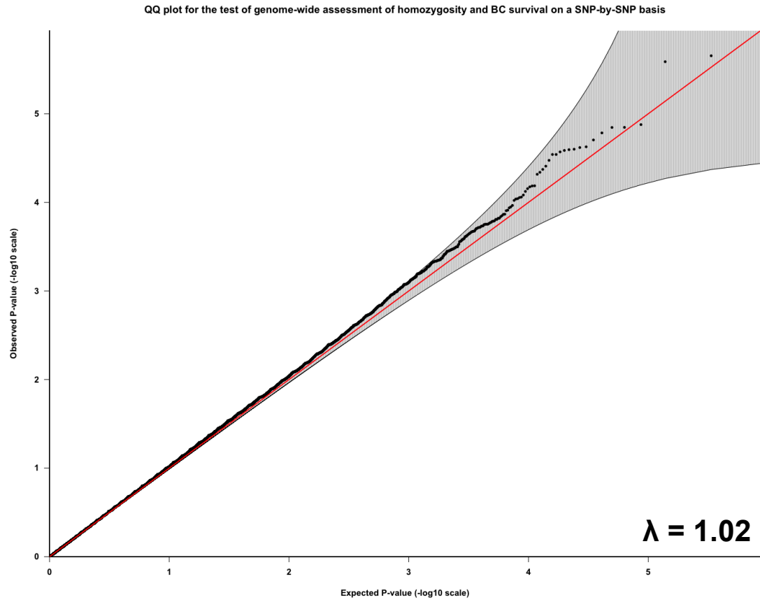
Supplemental Figure 1: QQ plot for the test of genome-wide assessment of homozygosity and BC survival on a SNP-by-SNP basis with a lambda ( \lambda ) = 1.02
