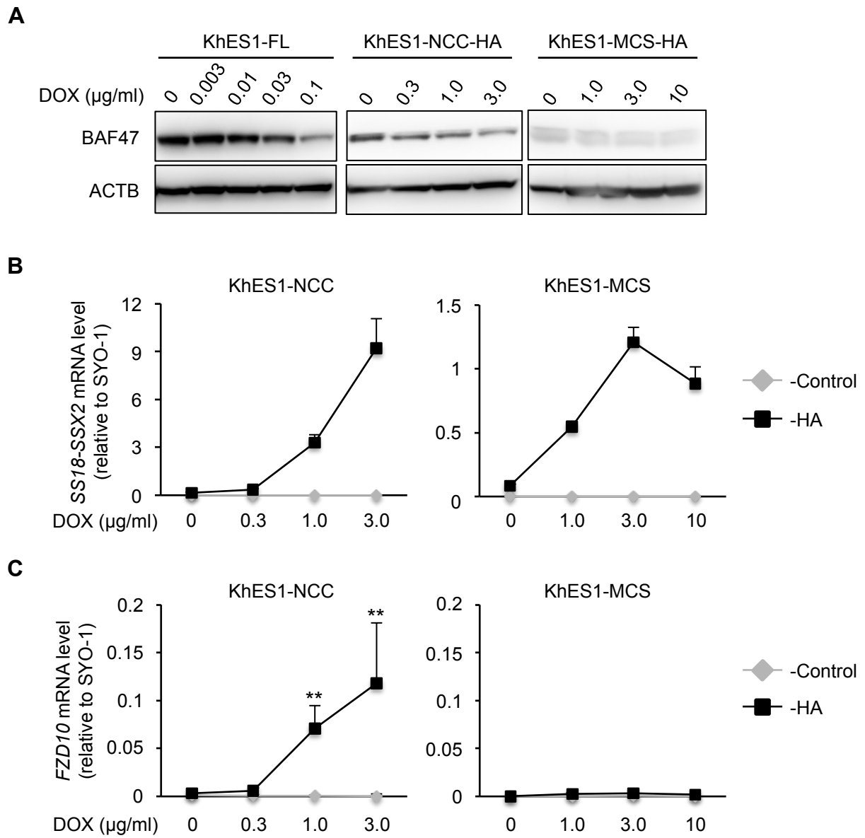
S6 Fig. Relationship between BAF47 levels and the induction of FZD10 .
