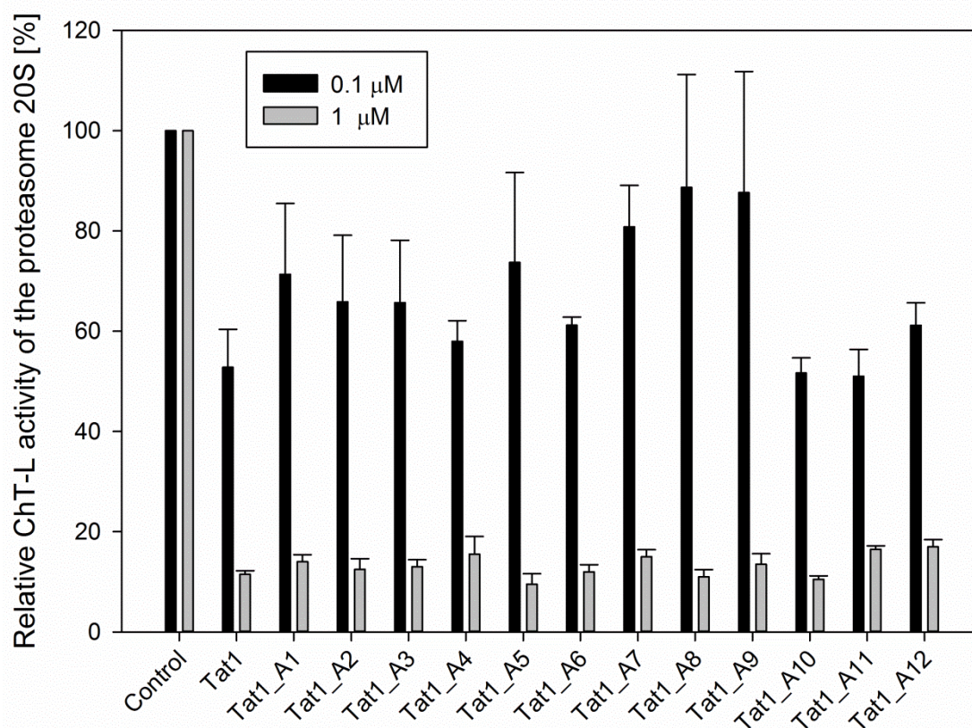
S1 Fig. Relative chymotrypsin-like activity of human 20S proteasome in the presence of Tat1 inhibitor or its Ala-scan analogs. The peptides concentration was either 0.1 or 1 \mu\text{M} .
