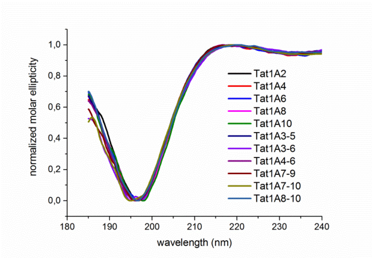
S5 Fig. Normalized CD spectra in water for the selected peptides with single and multiple Ala substitutions.
