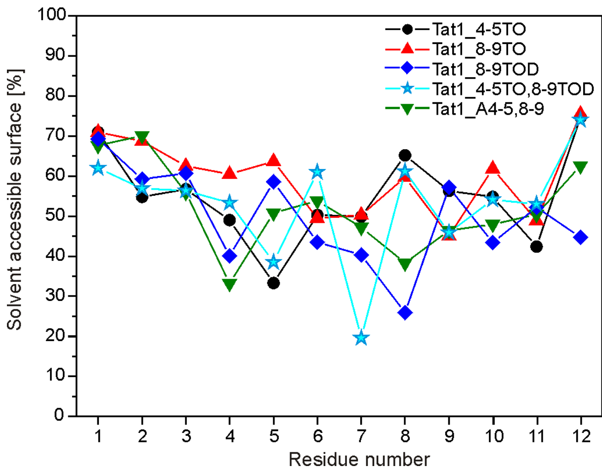
S8 Fig. The average surface accessibility of amino acid residues in the peptides studied calculated with MOLMOL using a solvent probe radius of 1.4 Å. The conformations obtained in the last 800 ps of MD simulations with time-averaged distance restraints and dihedral angle restraints.
