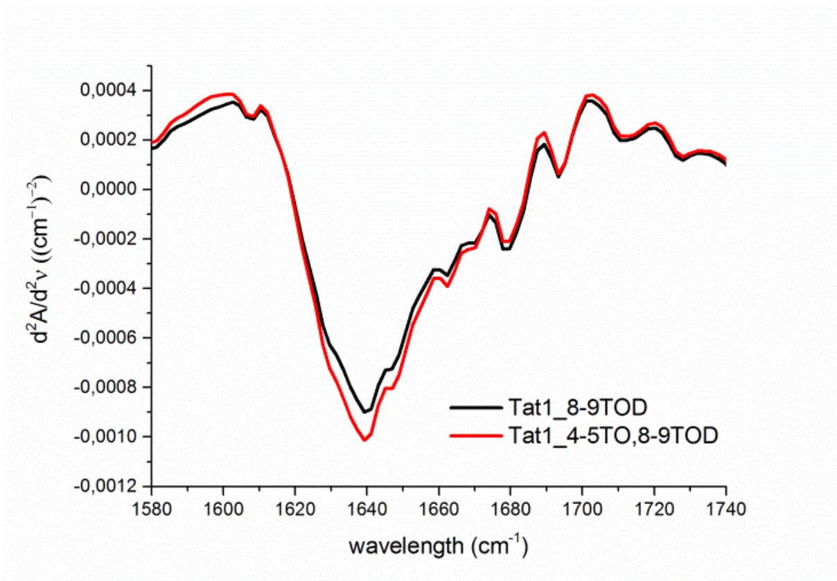
S9 Fig. Second derivative of Tat1_8-9TOD and Tat1_4-5TO,8-9TOD FTIR spectra recorded in water.
