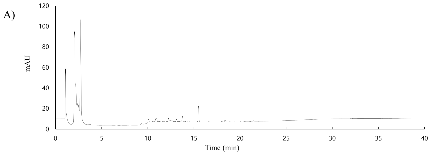
Supplementary figure 1. HPLC fingerprintings of ARA extract and Atractylenolide III
