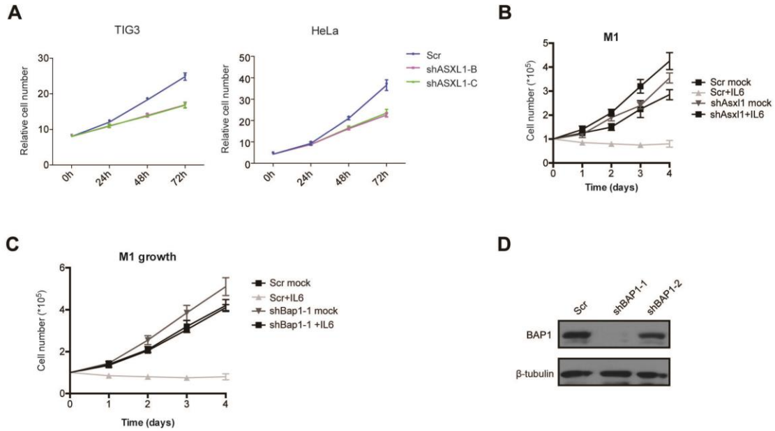
Supplementary information, Figure S6 Depletion of ASXL1 inhibits cell growth. (A) Growth curves of ASXL1-depleted TIG3, HeLa cells (shASXL1-B and shASXL1-C) compared with controls (Scr). (B-C) Growth curves of Asx11 or Bap1-depleted M1 cells (shAsx11, shBap1-1) compared with controls (Scr), untreated (mock) or treated by IL6 at the indicated times. The error bars denote s.d., n=2. (D) WB analysis confirmed the downregulation of BAP1 in BAP1-depleted (shBAP1-1 and -2) 293 cells. \beta -tubulin was used as loading control.
