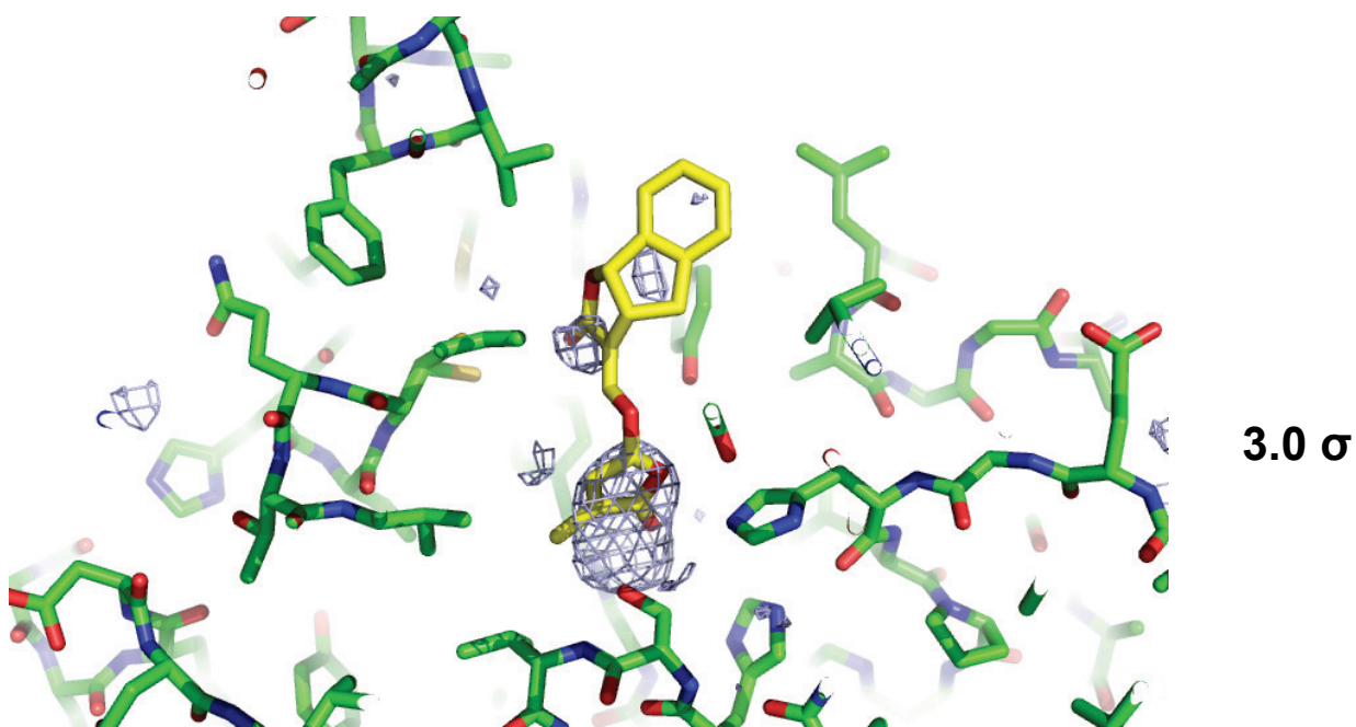
Supplementary information, Figure S1 Fo-Fc electron density maps calculated from the GR24 deleted model, contoured at 2 \sigma (top) or 3 \sigma (bottom).
