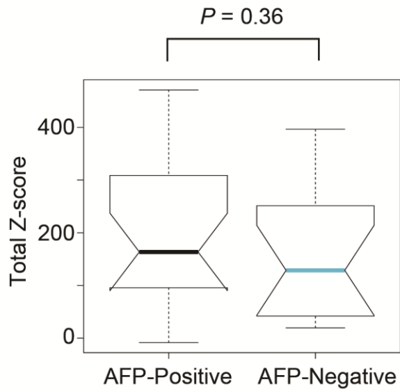
Figure S18. Methylation marker and AFP Comparison.
