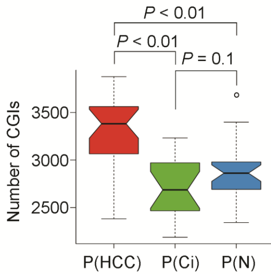
Figure S9. The number of CGI loci detected in plasma cfDNA.
