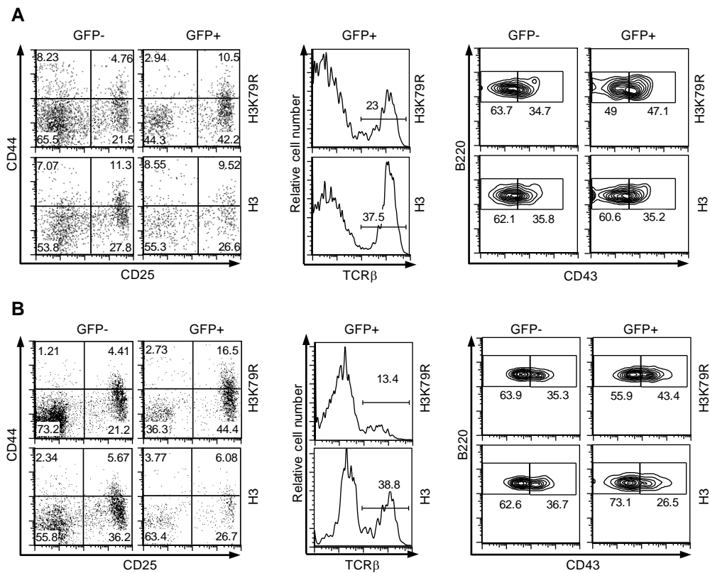
Supplementary Figure S3. Two additional repeats of the bone marrow transfer experiment in Figure 4. (A, B) The development of DN thymocytes (TCR \beta expression in DN3 thymocytes) and early B cells transfected with indicated mutant histone H3 were assessed by flow cytometry.
