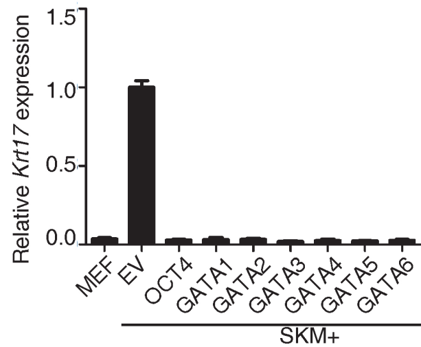
Supplementary Information, Figure S2 Quantitative RT-PCR analysis of the expression of endogenous ECT related genes relative to the expression of SKM.
