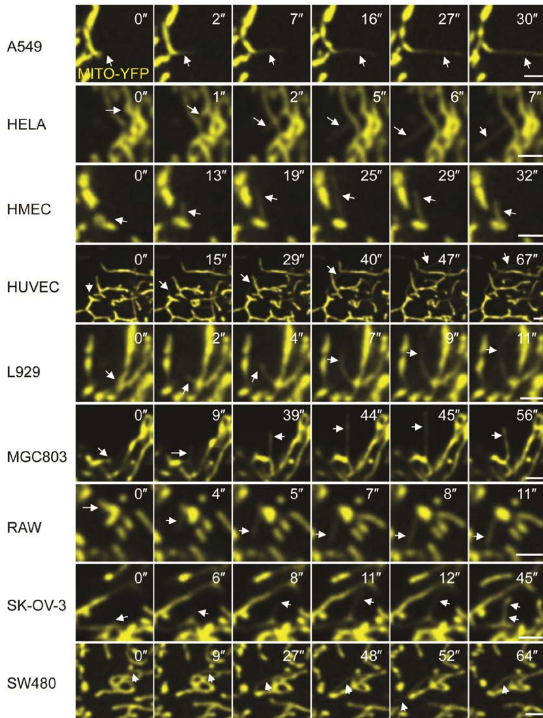
Figure S3 Dynamic tubulation of mitochondria is a common phenomenon in different cell lines. The indicated cell lines were transfected with Mito-YFP and observed with a spinning-disk microscope system. Scale bar, 2 \mu m. Structures indicated by the white arrows are dynamic tubules.
