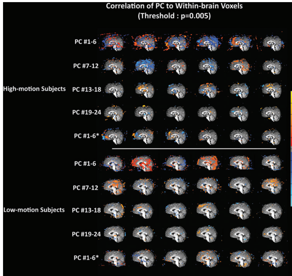
SUPPLEMENTARY FIG. S1. Spatial distribution of areas significantly correlated with the principal components (PCs). The PCs were correlated to each voxel time series for each of the motion correction methods. The maps were thresholded at p=0.005 . * indicates PCs derived after \delta_{mot} and used in the \delta_{mot\delta edge}^* model.
