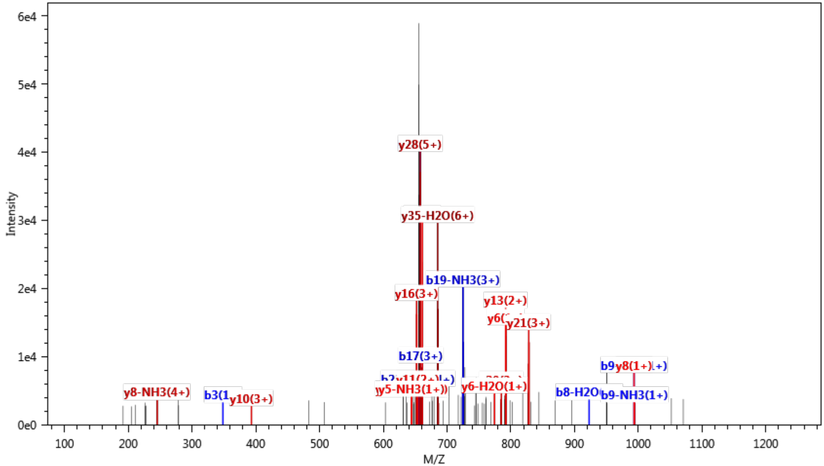
Ms2 Spectrum (Scan: 8379, Raw: CPTAC_OT_Pep_JB_5429_5min_4May12_Legolas_11-07-64)
