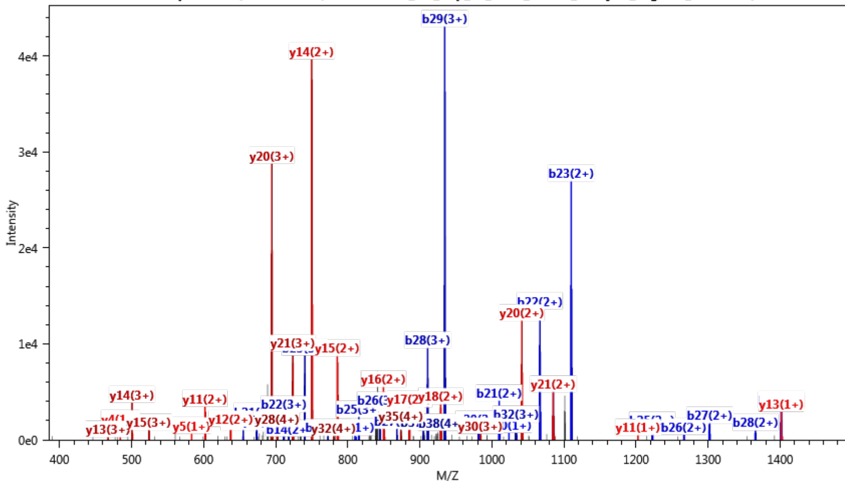
Ms2 Spectrum (Scan: 10414, Raw: CPTAC_OT_Pep_JB_5429_60min_4May12_Legolas_11-07-64)
