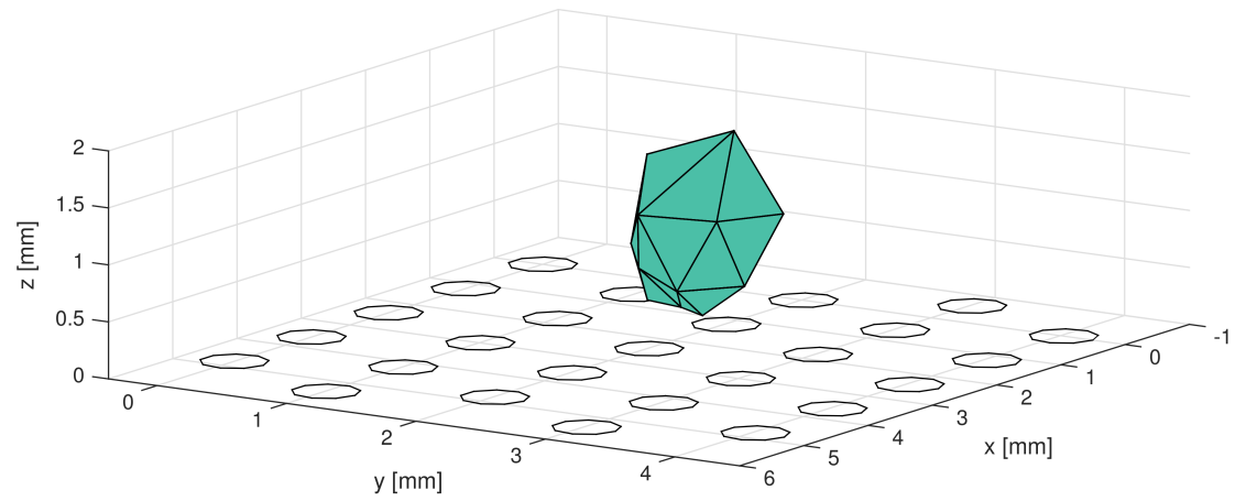
Supplementary Figure 1. Reconstruction of 1-mm-diameter glass bead placed 1 mm away from the electrode array. The glass bead appeared as a region of higher impedance than the saline background. Image shows the electrodes (black circles) and the voxels (cyan) with impedance changes ( dZ ) greater than 50%.
