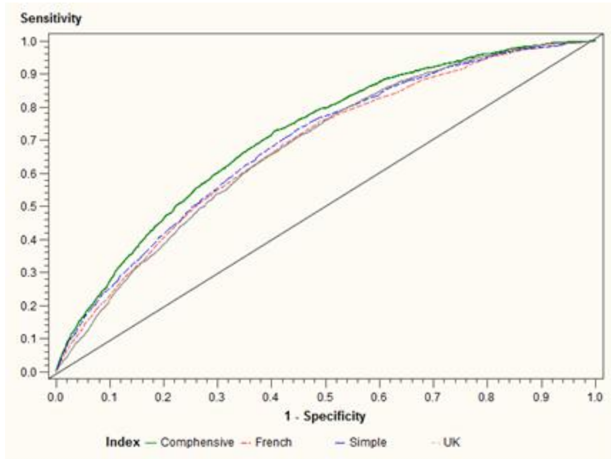
Figure S1. Receiver operating characteristic curves for different models: validation cohort.
