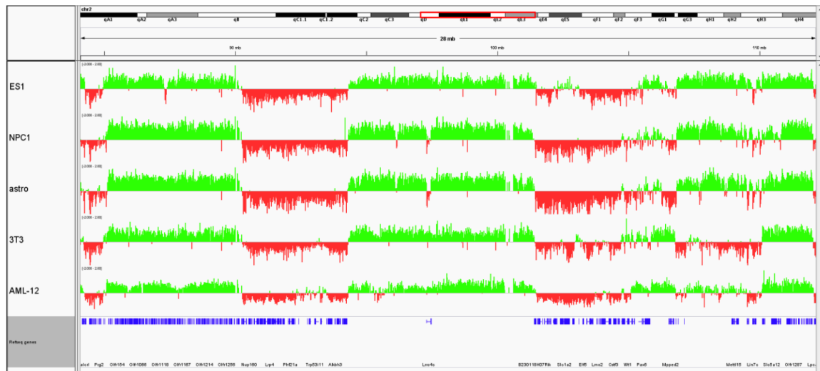
Figure S3. Comparison of LMNB1-chromatin association maps among cell types. Showing is LMNB1 signals of embryonic stem cells (ES), neural progenitor cells (NPC), Astrocytes (Astro), 3T3 cells and AML12 cells, on a 28 Mb region of chromosome 2.
