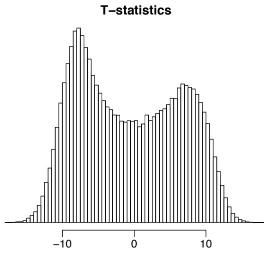
Figure S2. Histogram of probe level t-statistics from smoothed signals. Histogram of the resulting test statistics shows a clear bimodal distribution. Two parts of the distribution represent probes from Lamin B1 associated chromatin domains (LADs) and non-LADs.
