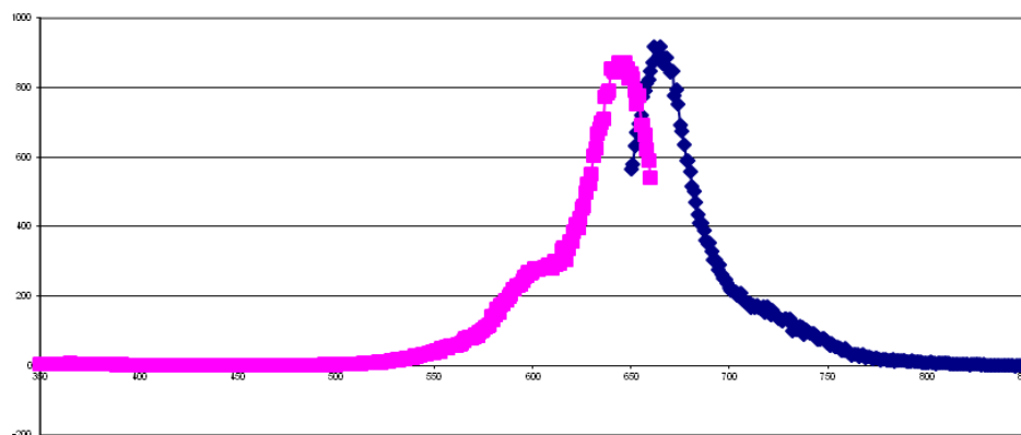
Fluorescence spectrum of compound 3
