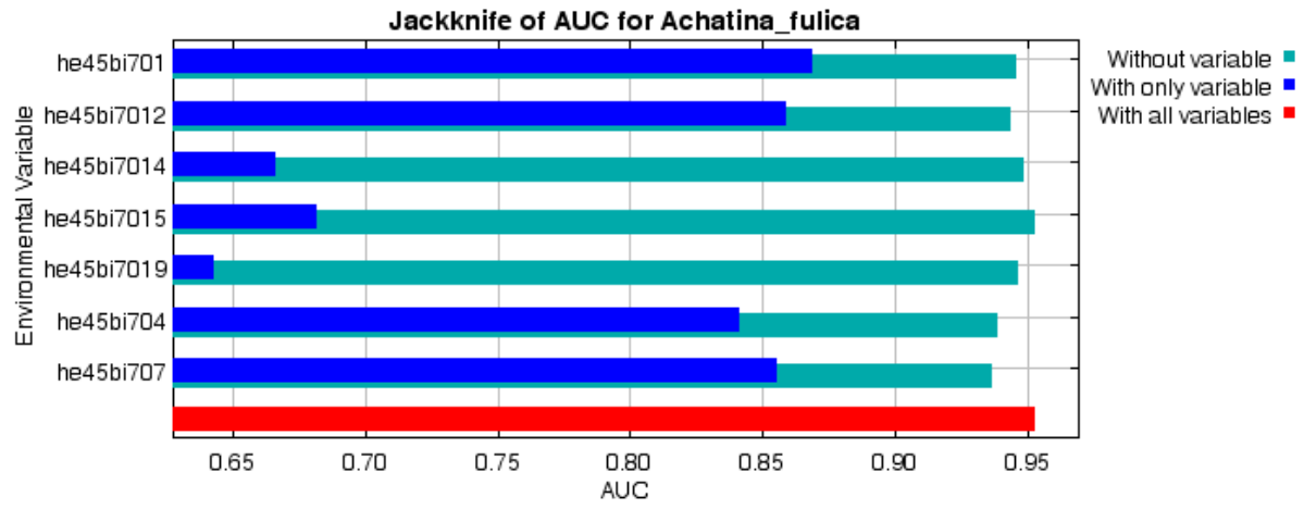
S2 Fig: Jackknife test of variable importance for A.fulica under RCP 4.5 scenario
