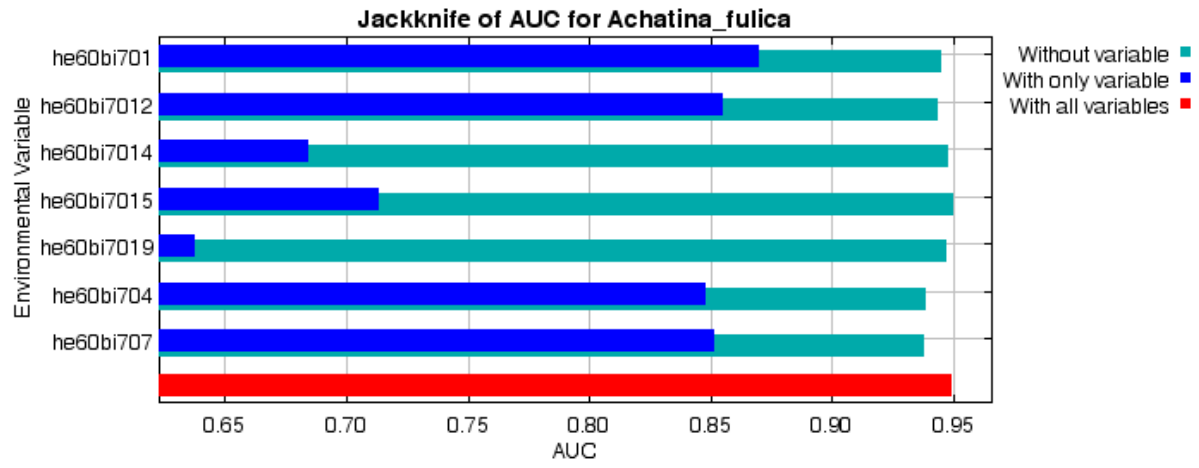
S3 Fig: Jackknife test of variable importance for A.fulica under RCP 6.0 scenario
