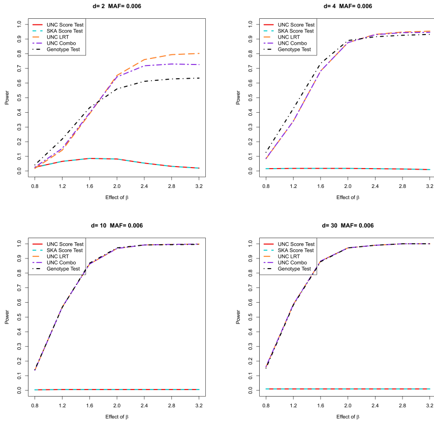
Supplementary Figure 1: Powers of single SNP testing for quantitative trait with p_{\text{threshold}} = 0.01 , \text{MAF} = 0.006 and n = 1000 .
