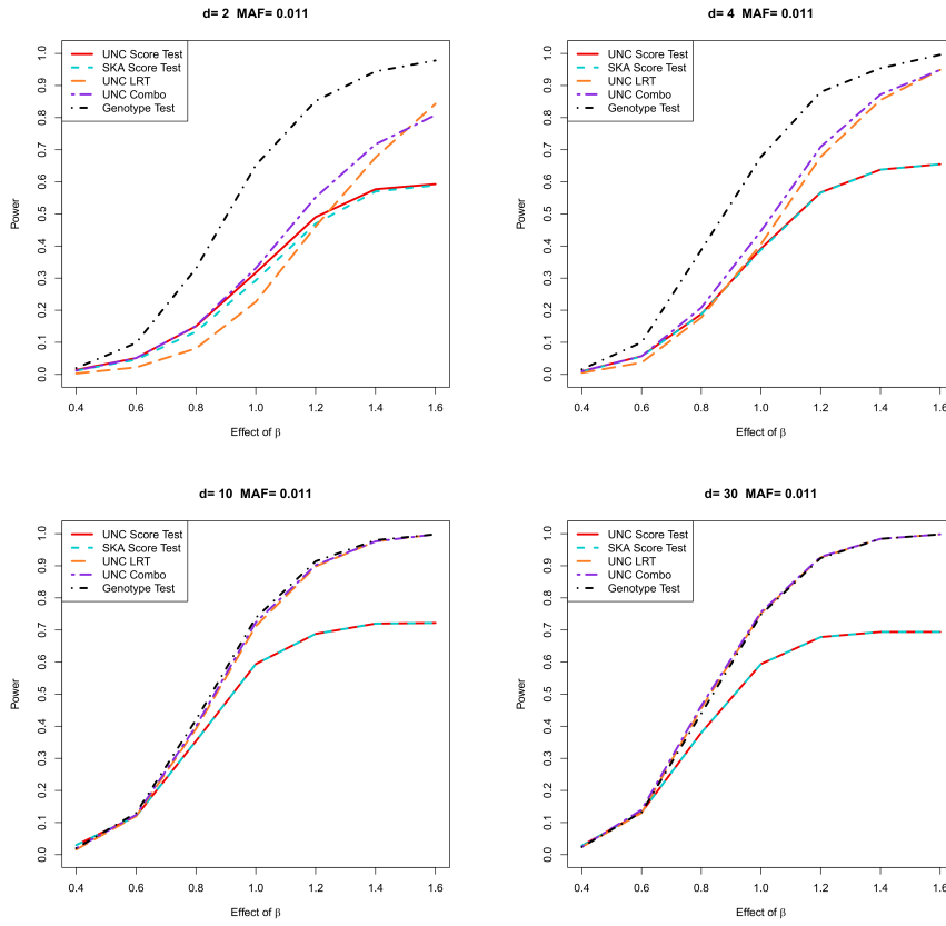
Supplementary Figure 2: Powers of single SNP testing for quantitative trait with p_{\text{threshold}} = 0.01 , \text{MAF} = 0.011 and n = 1000 .
