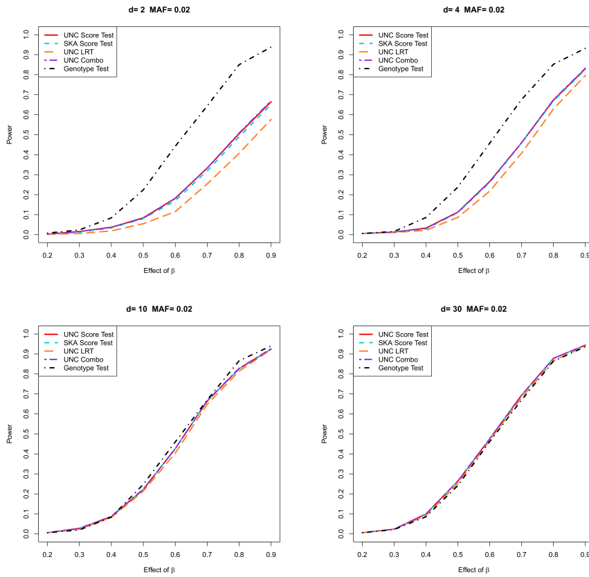
Supplementary Figure 3: Powers of single SNP testing for quantitative trait with p_{\text{threshold}} = 0.01 , \text{MAF} = 0.02 and n = 1000 .
