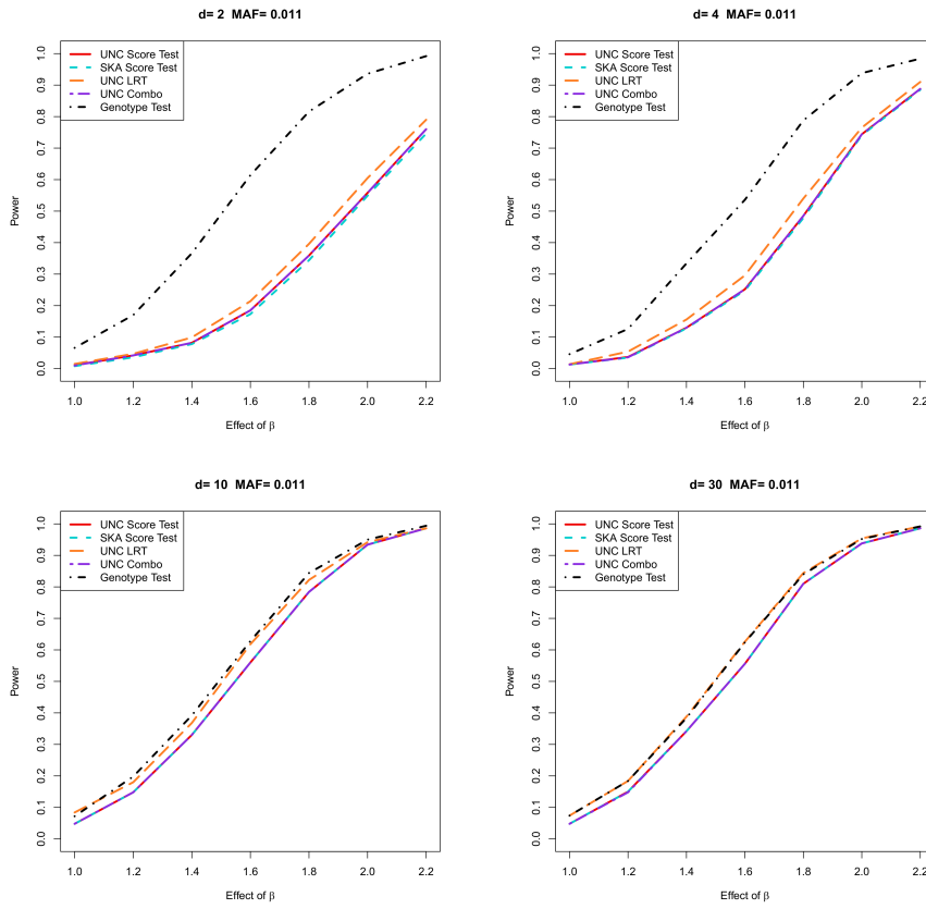
Supplementary Figure 5: Powers of single SNP testing for binary trait with p_{threshold} = 0.01 , MAF=0.011 and n = 1000 .
