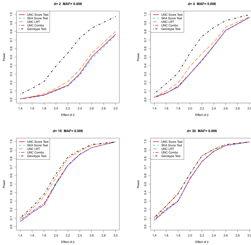
Supplementary Figure 4: Powers of single SNP testing for binary trait with p_{threshold} = 0.01 , MAF=0.006 and n = 1000 .
