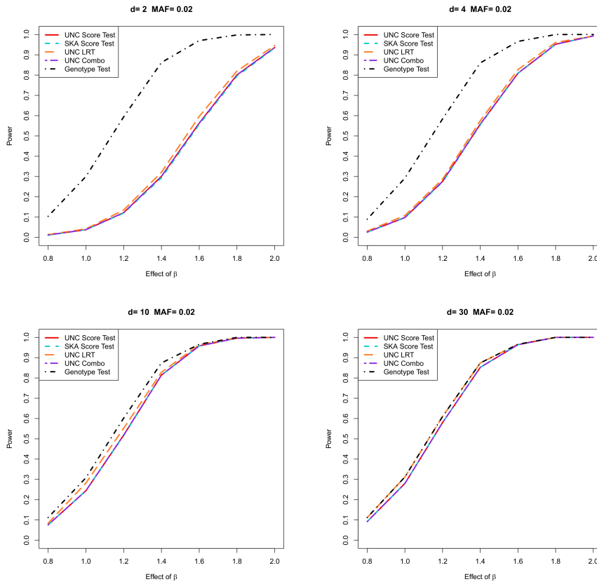
Supplementary Figure 6: Powers of single SNP testing for binary trait with p_{threshold} = 0.01 , MAF=0.02 and n = 1000 .
