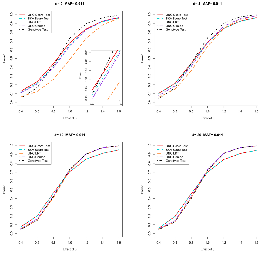
Supplementary Figure 7: Powers of multiple testing for quantitative trait with p_{\text{threshold}} = 0.01 , \text{MAF} = 0.011 and n = 1000 .
