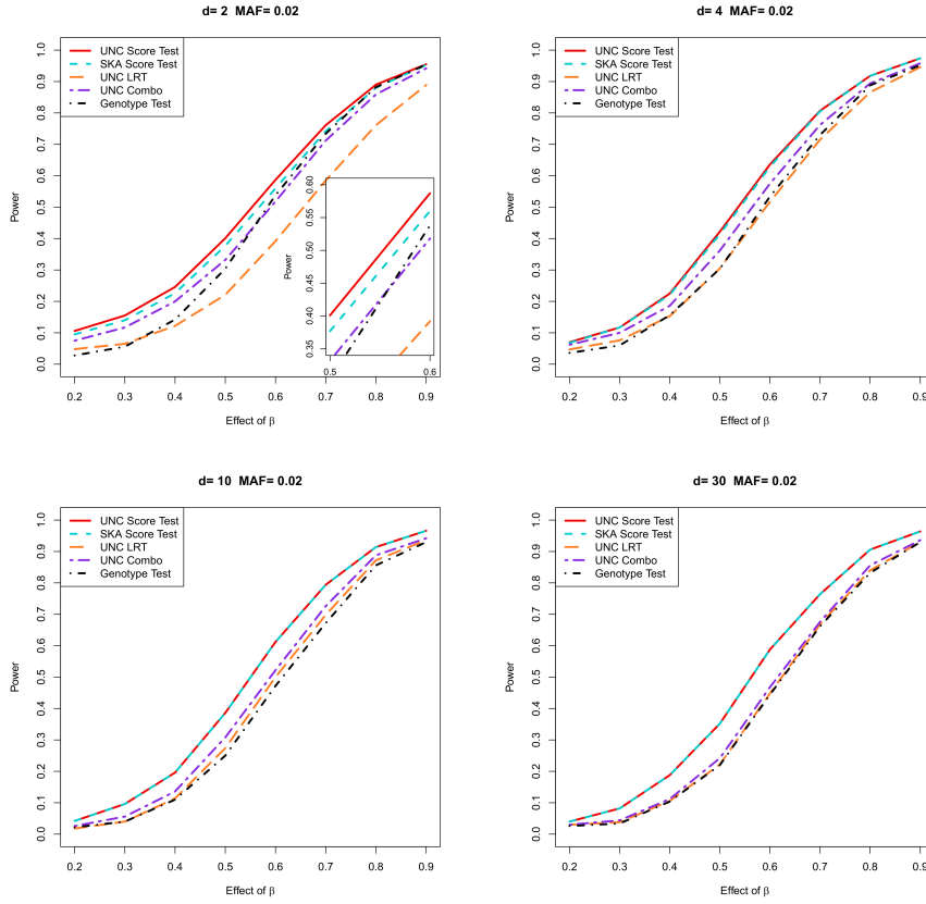
Supplementary Figure 8: Powers of multiple testing for quantitative trait with p_{\text{threshold}} = 0.01 , \text{MAF} = 0.02 and n = 1000 .
