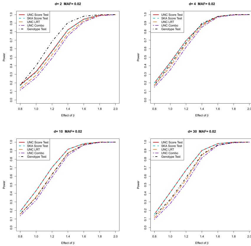
Supplementary Figure 11: Powers of multiple testing for binary trait with p_{threshold} = 0.01 , MAF=0.02 and n = 1000 .
