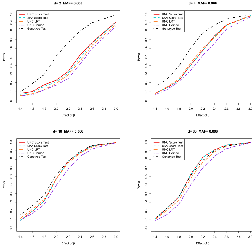
Supplementary Figure 9: Powers of multiple testing for binary trait with p_{threshold} = 0.01 , MAF=0.006 and n = 1000 .
