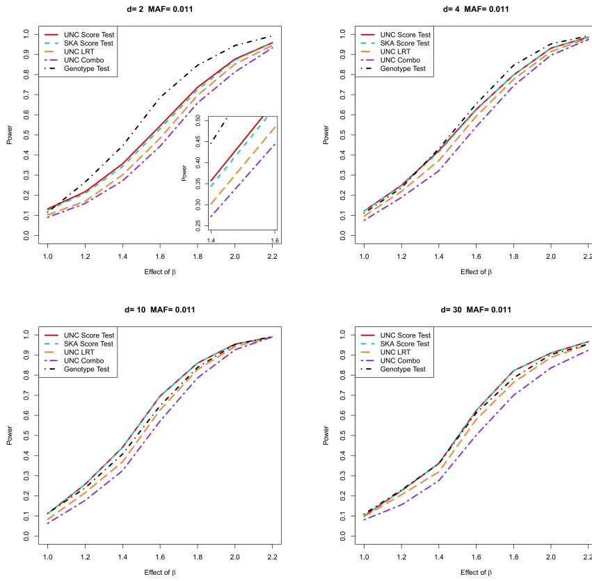
Supplementary Figure 10: Powers of multiple testing for binary trait with p_{threshold} = 0.01 , MAF=0.011 and n = 1000 .
