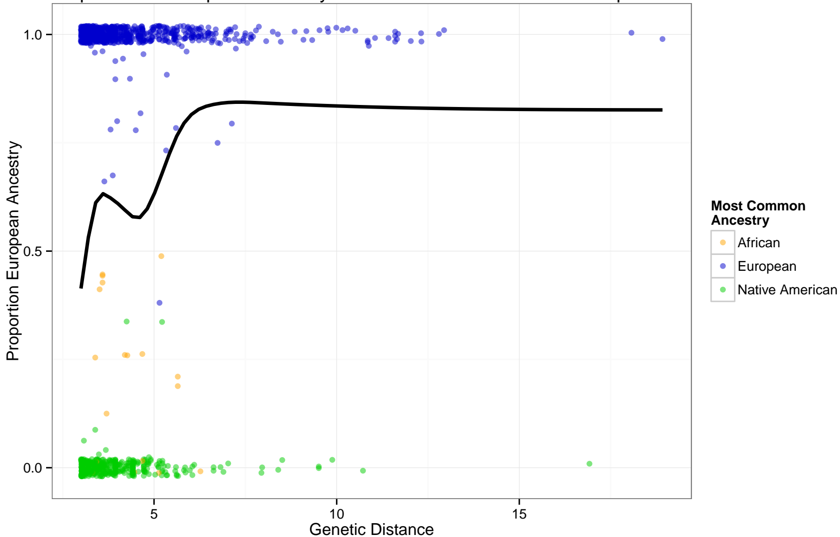
Proportion of European Ancestry in IBD Tracts Shared Between Populations
