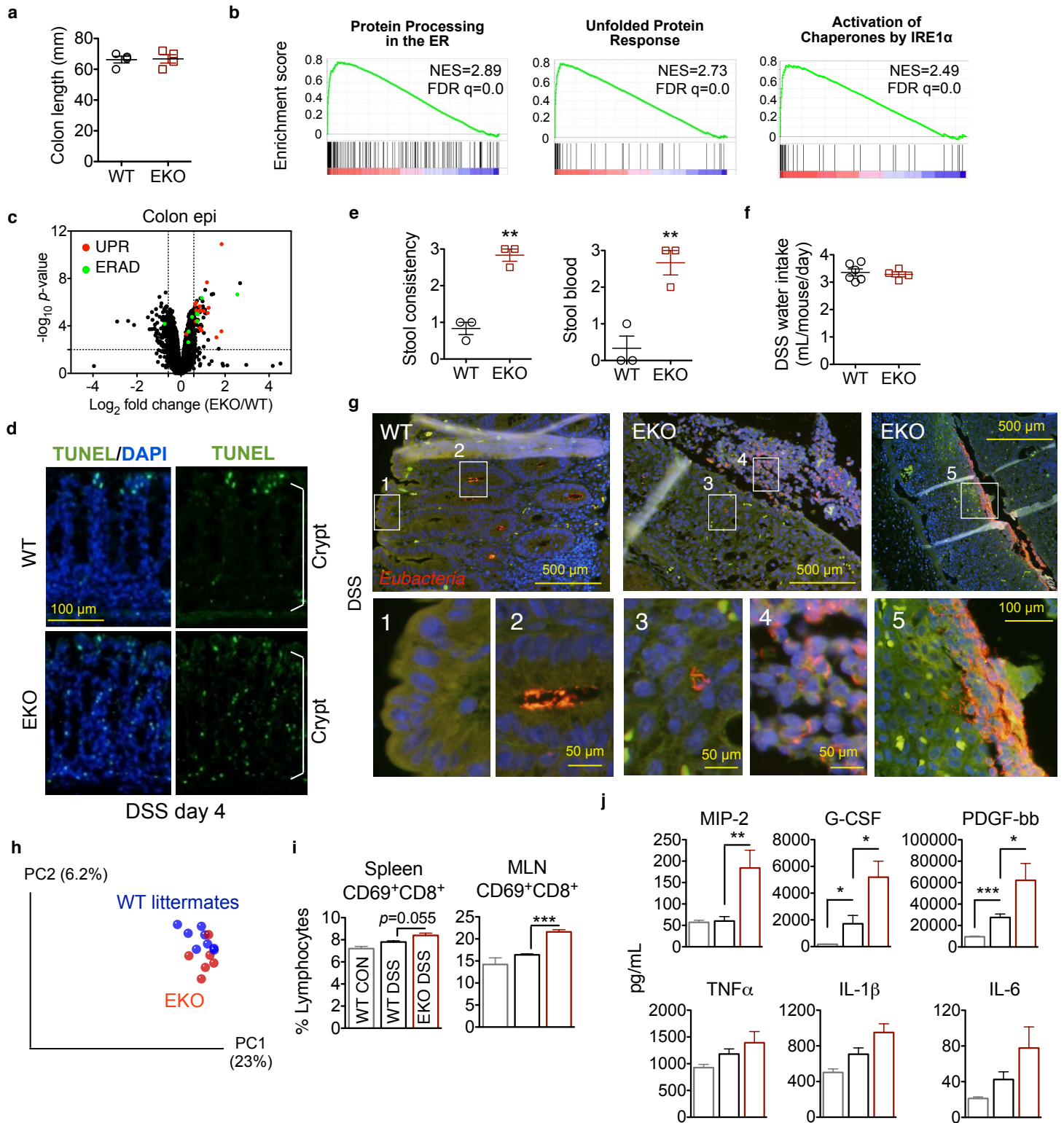
Supplementary Figure 5. The status of UPR and IRE1 \alpha signaling in colonic epithelium and sensitivity to experimental colitis of Sei1L \Delta IEC (EKO) mice.
