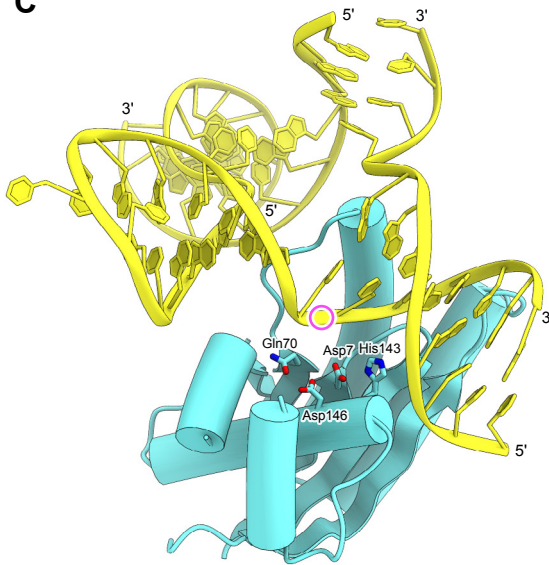
T. thermophilus RuvC–substrate DNA (PDB ID 4LD0)
