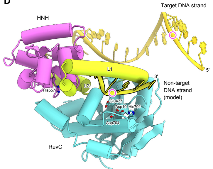
SaCas9–sgRNA–target DNA–non-target DNA (model)
