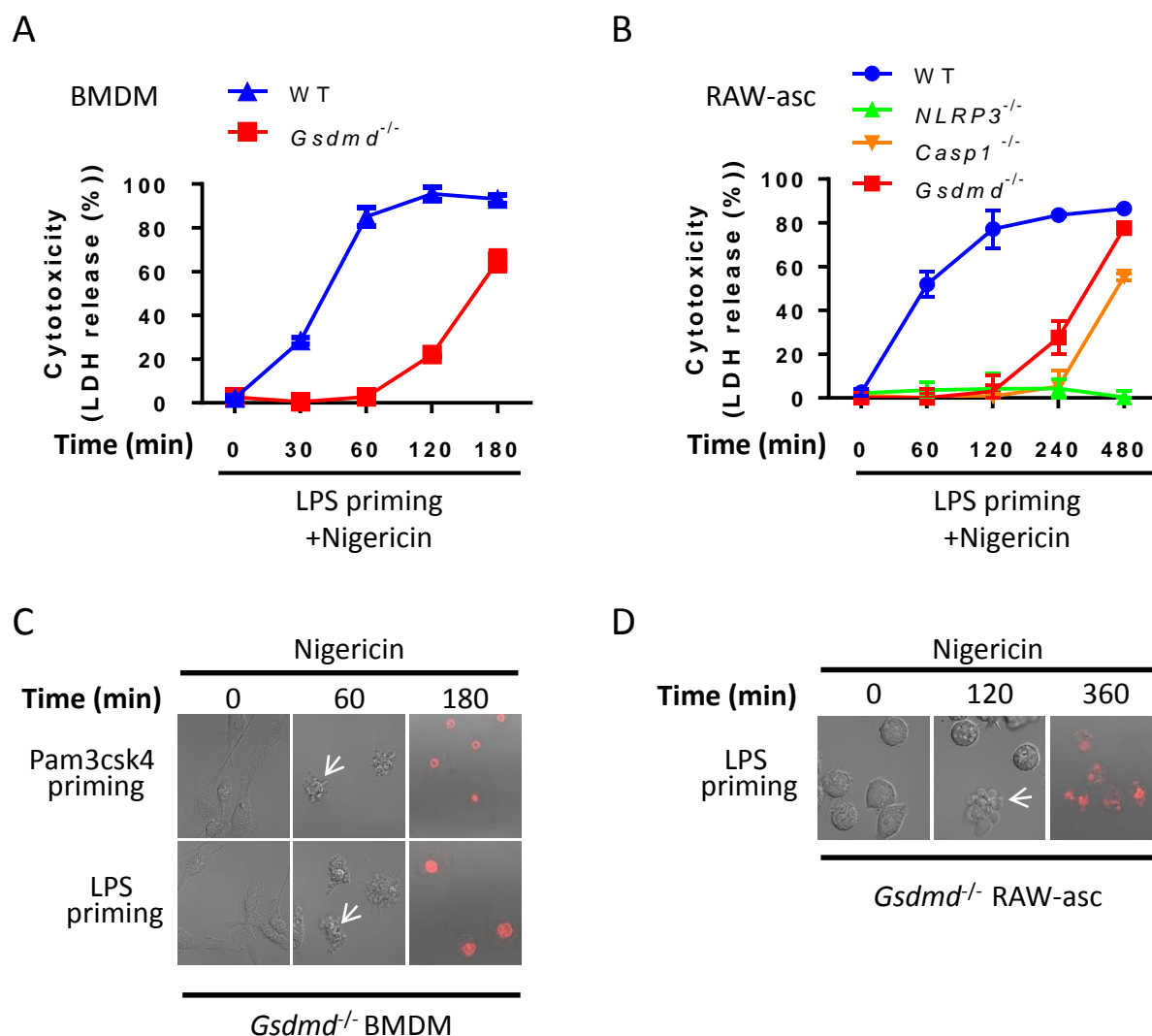
Figure S4. Secondary necrosis of apoptotic cells in inflammasome stimuli-treated Gsdmd -/- cells. A. WT and Gsdmd -/- BMDM were primed with LPS for 4 hours and stimulated with nigericin for different periods of time as indicated. LDH release was measured and shown. B. The same as in A except that WT and Gsdmd -/- RAW-asc cells were used. C. WT and Gsdmd -/- BMDM were primed with Pam3csk4 for 5 hours or LPS for 4 hours and then stimulated with nigericin for different periods of time as indicated. Images were taken at the time points indicated. D. WT and Gsdmd -/- RAW-asc cells were primed with LPS for 4 hours and stimulated with nigericin for different periods of time as indicated. Images were taken at the time points indicated.
