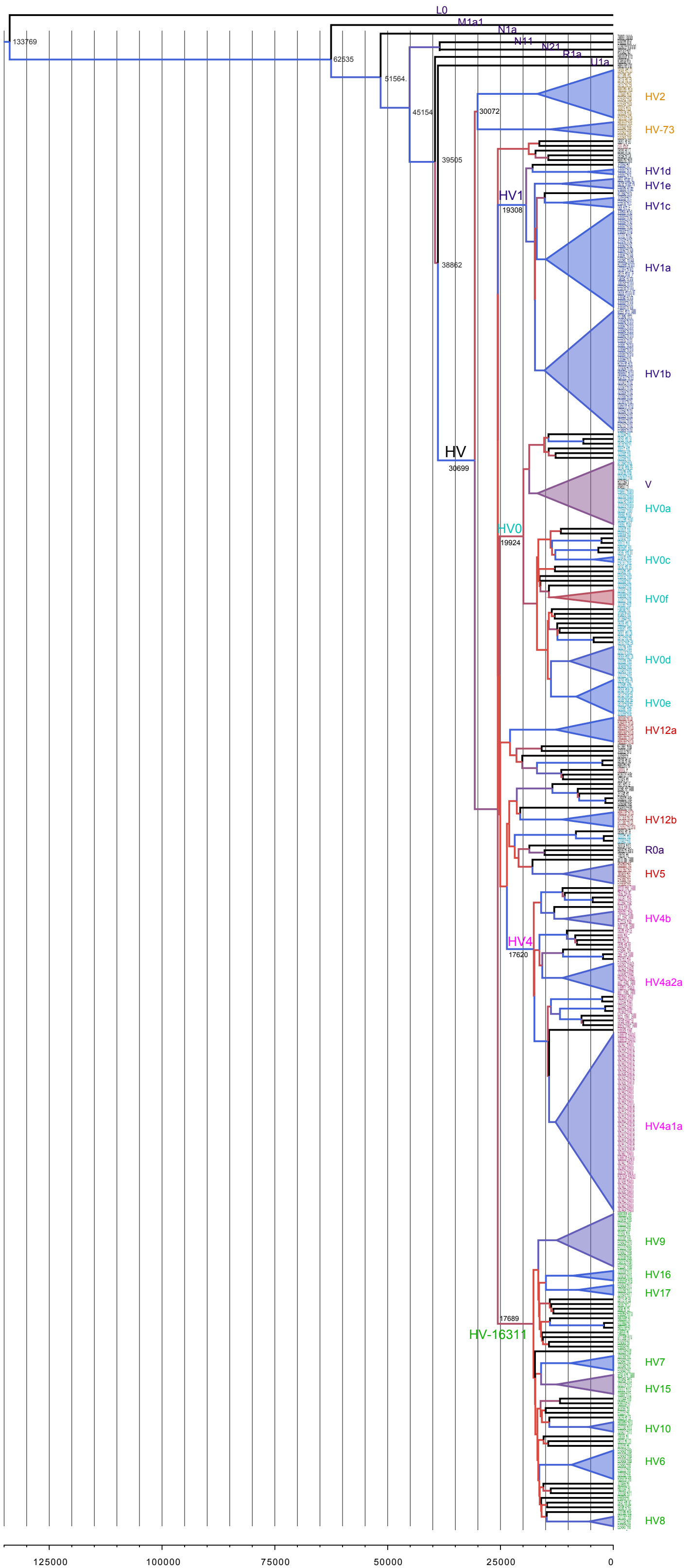
S2 Fig. Phylogenetic tree with all the 316 sequences of the dataset. Realized in BEAST.
