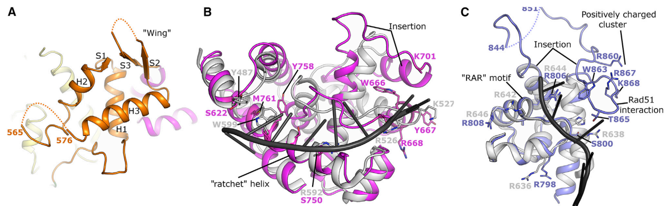
Figure 2. Structure and Comparison of Pol \theta -HLD Domains 3 to 5
