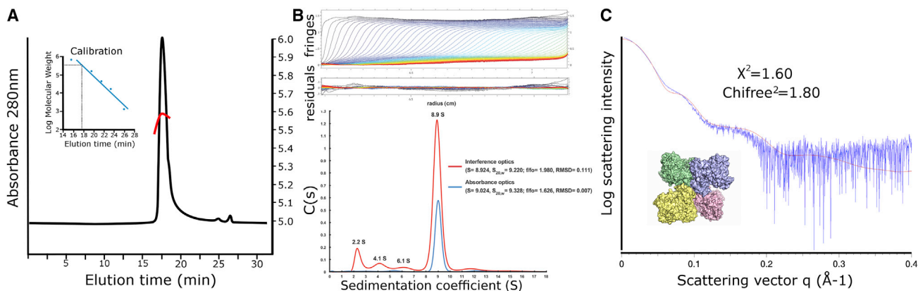
Figure 4. Analysis of Pol \theta -HLD in Solution
