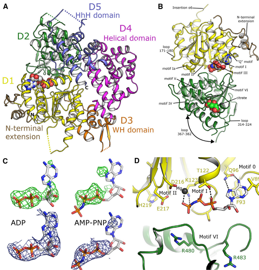
Figure 1. Structure of Pol \theta -HLD and ATPase Core
