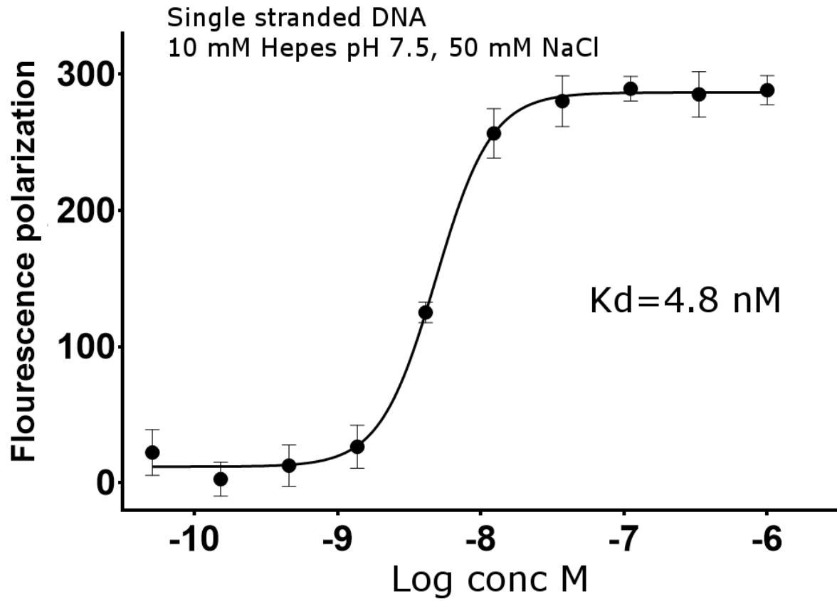
Figure S3, related to Figure 5- Polθ-HLD binding to single stranded DNA in low salt buffer. Error bars are plotted \pm standard error of at least three independent replicates.
