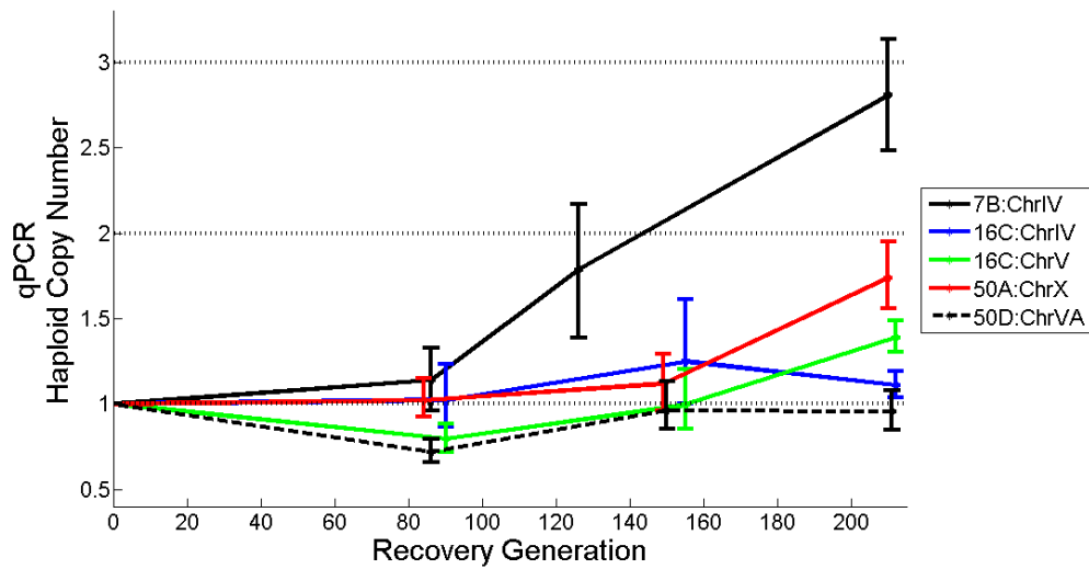
Supplemental Figure S3. Increase in the frequencies of five unique duplications that lack overlap in their duplication spans. Frequencies of five unique duplications in adaptive recovery populations 7B, 16C, 50A, and 50D. The average copy-number per haploid genome was calculated from qPCR results and is indicated on the vertical axis. The number of recovery generations is indicated on the horizontal axis.
