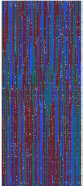
Chr8
