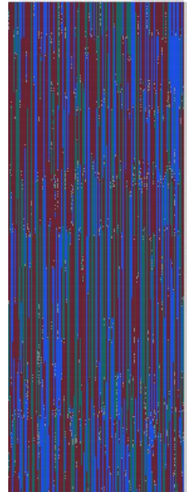
Chr12
