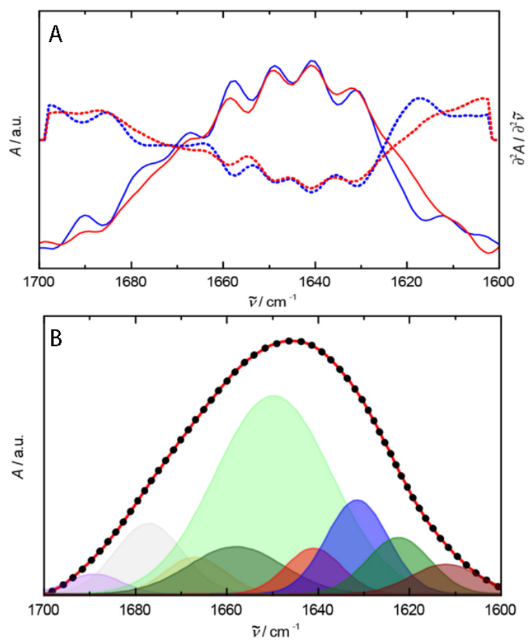
Fig. S 4 (A) FSD (solid lines) and 2 nd derivative (dashed lines) spectra of the amide I' band of MT1-MMP (pressure of 1 bar in blue and 11 kbar in red). (B) Amide I' band of MT1-MMP at 1 bar (black filled circles) and fitted curve (red line) generated by the superposition of the underlying Gaussian-shaped subbands.
