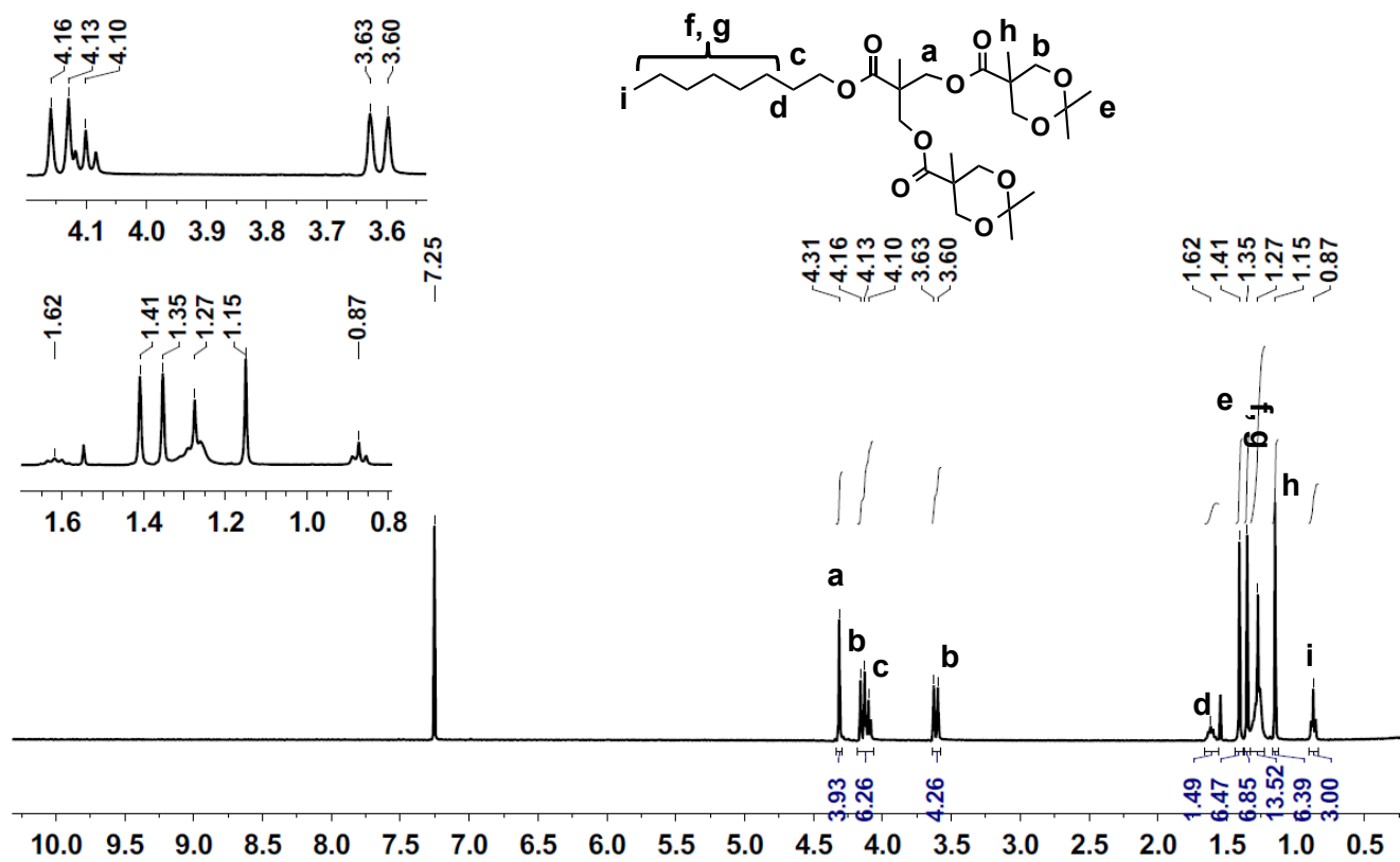
Figure S19. ^1\text{H} NMR of \text{Oc-[G2]-(An)}_2 (7) in \text{CDCl}_3 .
