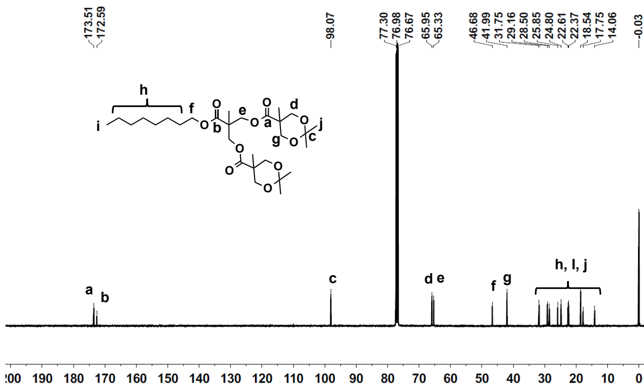
Figure S20. ^{13}\text{C} NMR of \text{Oc-[G2]-(An)}_2 (7) in \text{CDCl}_3 .
