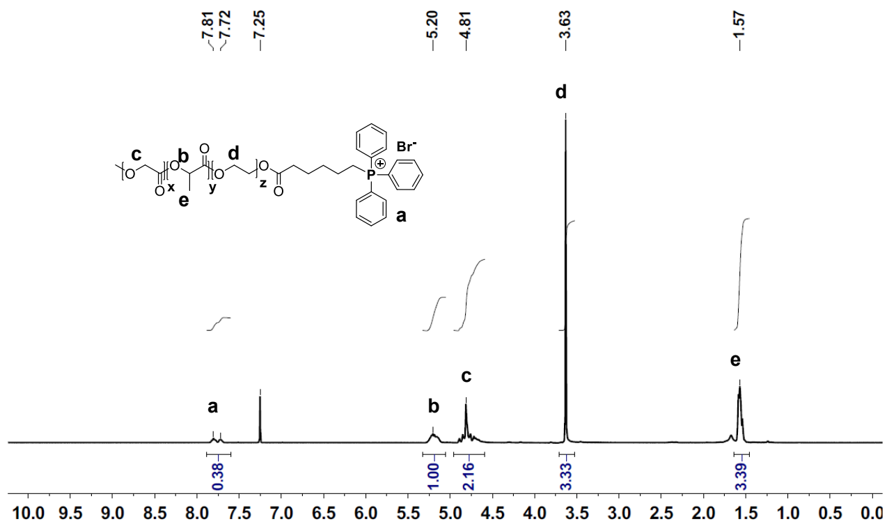
Figure S4. ^1\text{H} NMR of PLGA- b -PEG-TPP in \text{CDCl}_3 .
