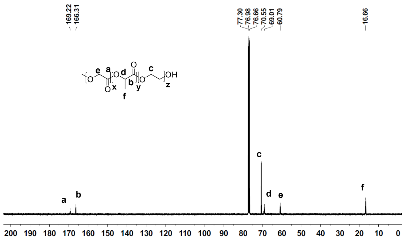
Figure S2. ^{13}\text{C} NMR of PLGA- b -PEG-OH in \text{CDCl}_3 .
