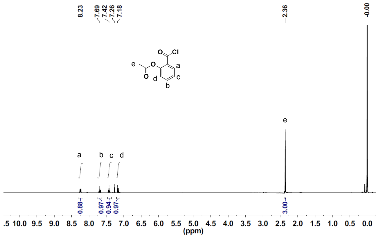
Figure S13. ^1\text{H} NMR of compound 5 in \text{CDCl}_3 .
