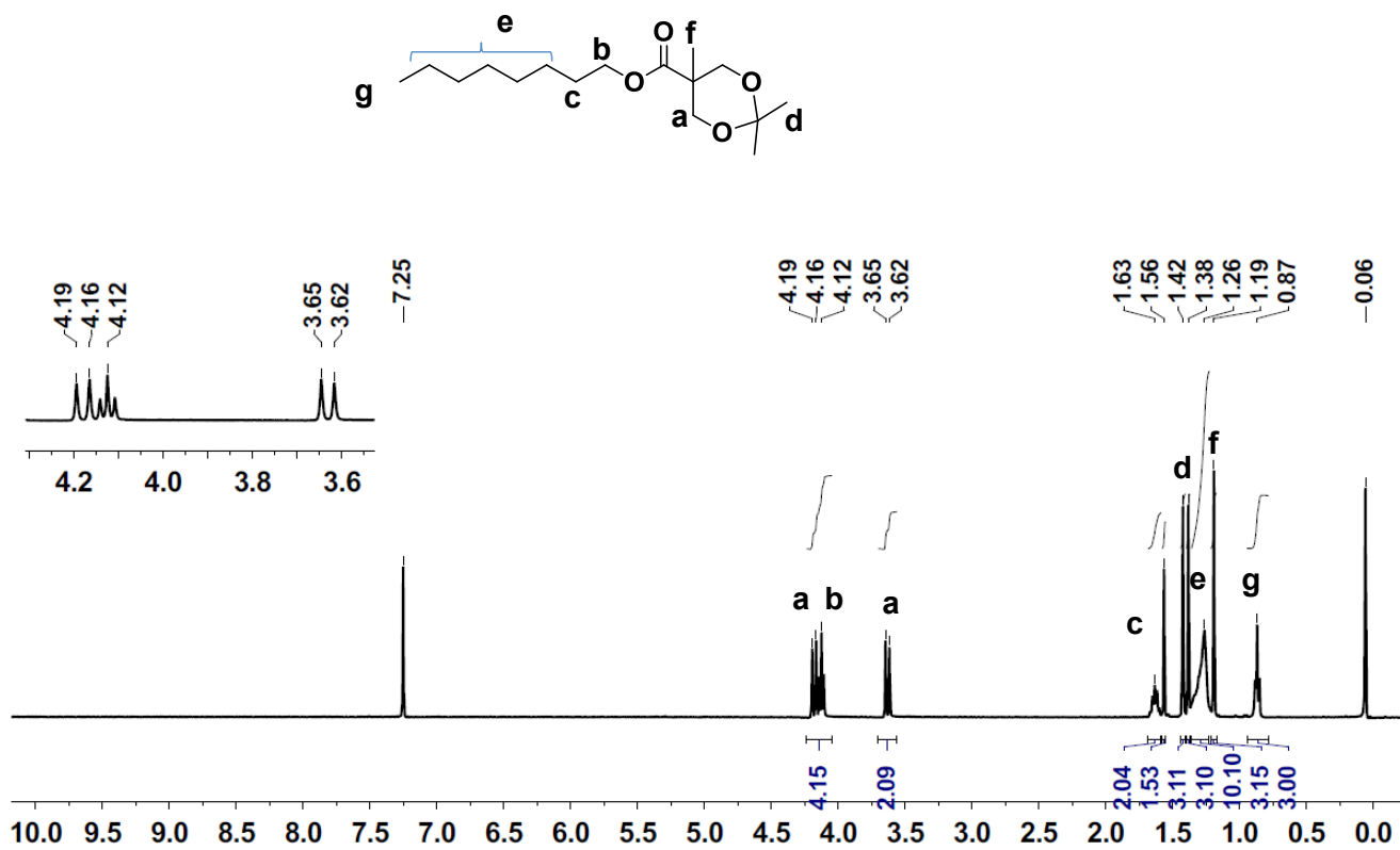
Figure S7. 1 H NMR of Oc-[G1]-An (3) in CDCl 3 .
