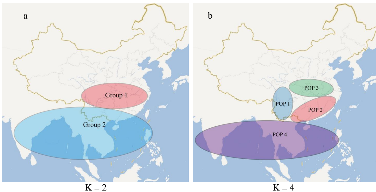
Figure S2 The geographic distribution of different subpopulations. (a) Two groups were inferred by STRUCTURE, K = 2 ; (b) Four subpopulations were inferred by STRUCTURE, K = 4 .
