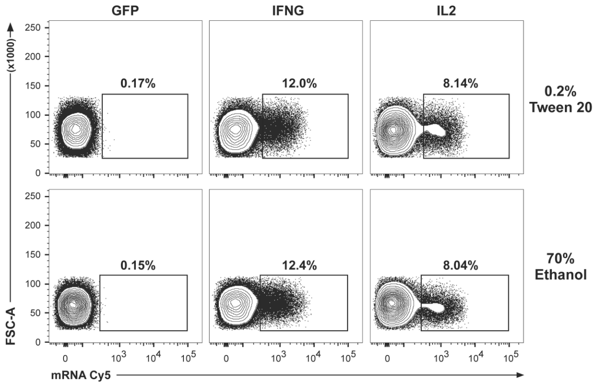
S4 Fig. Comparison of permeabilization buffers containing 70% ethanol or 0.2% Tween 20.
