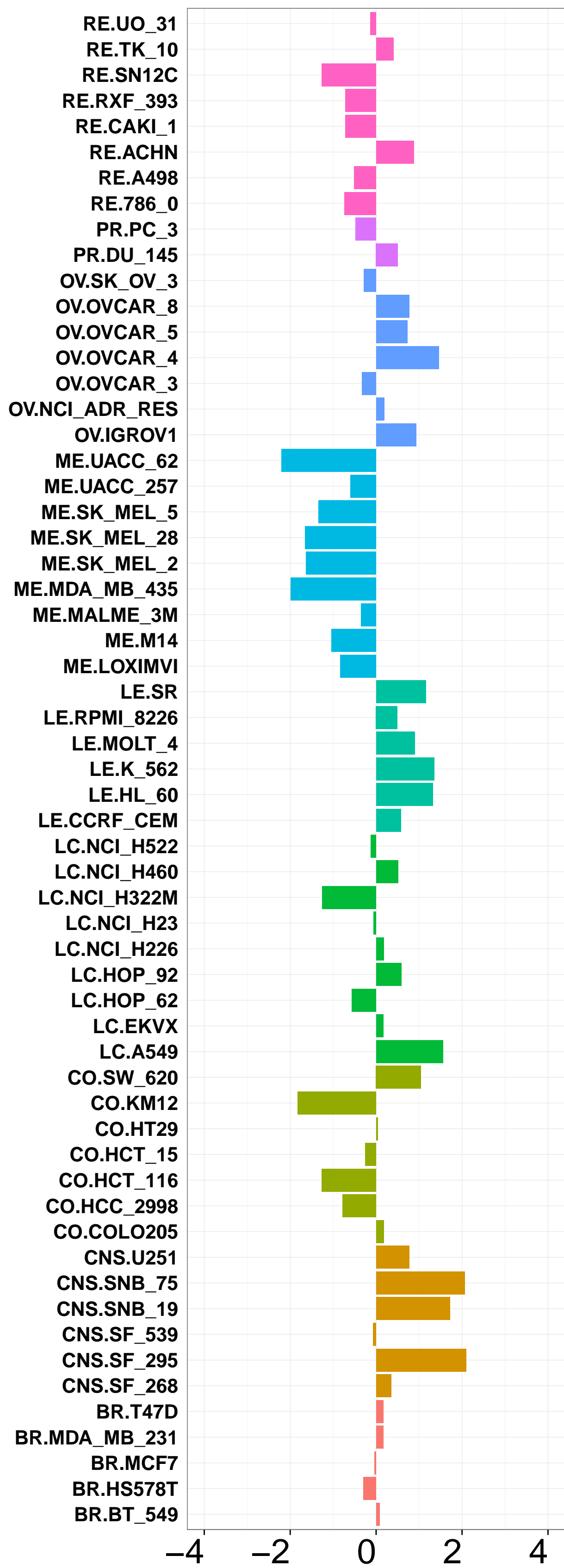
Predicted (Z-scores)
