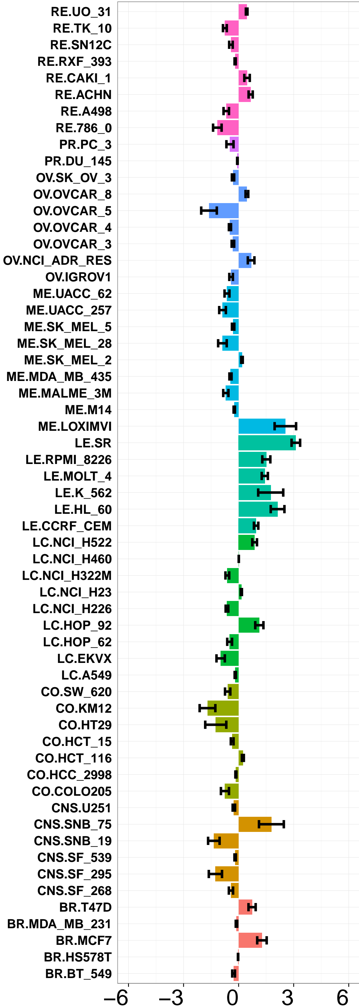
Predicted (Z-scores)
