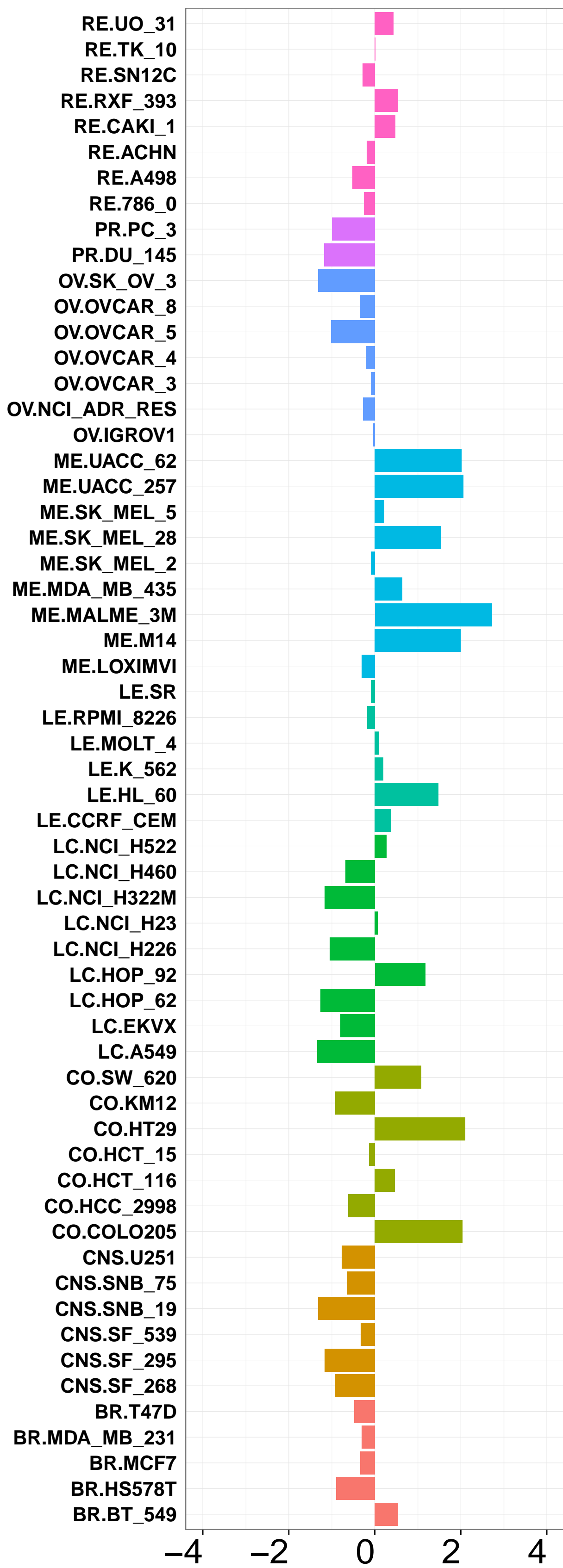
Observed (Z-scores)
