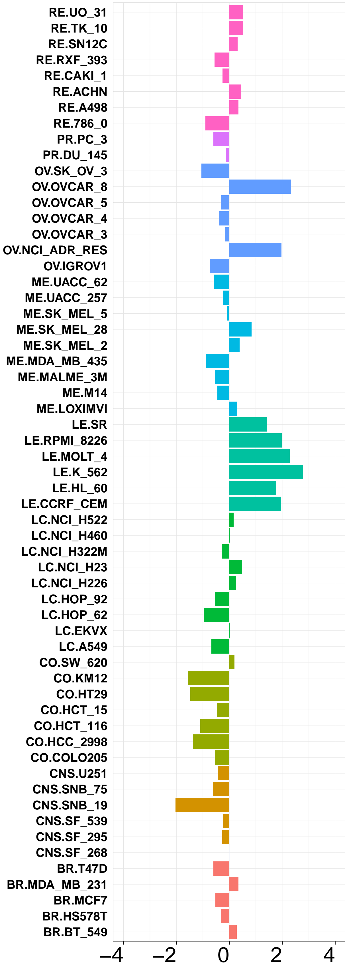
Predicted (Z-scores)
