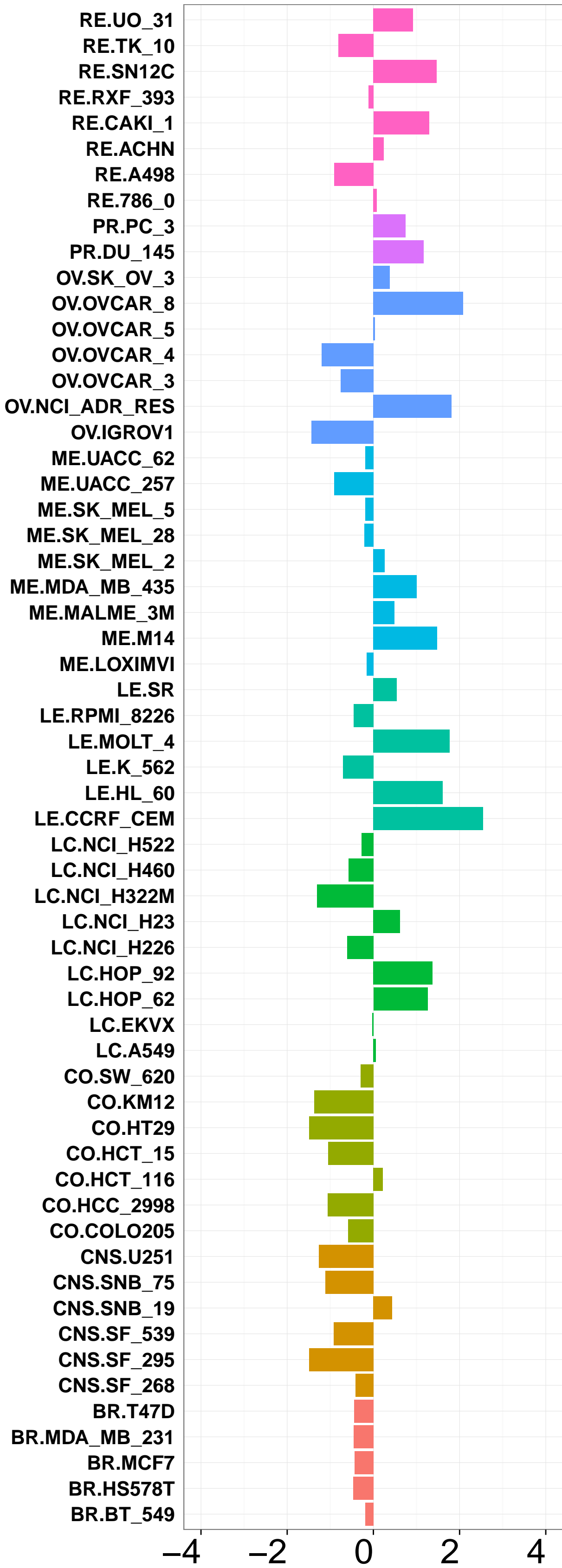
Observed (Z-scores)
