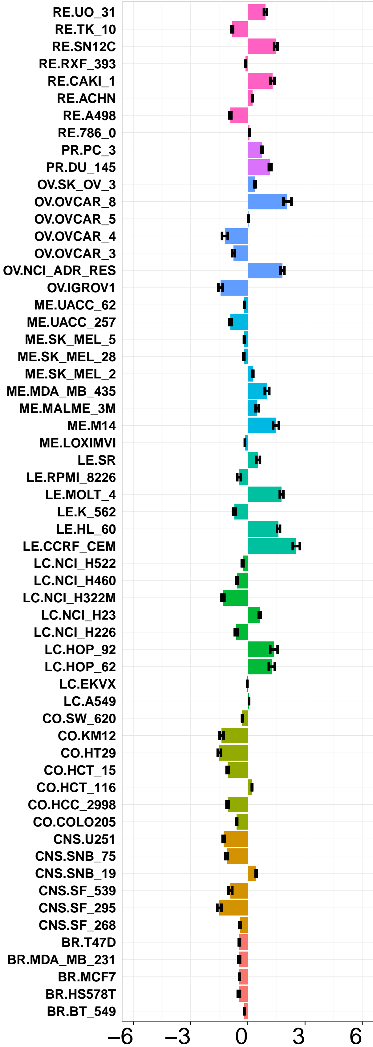
Observed (Z-scores)
