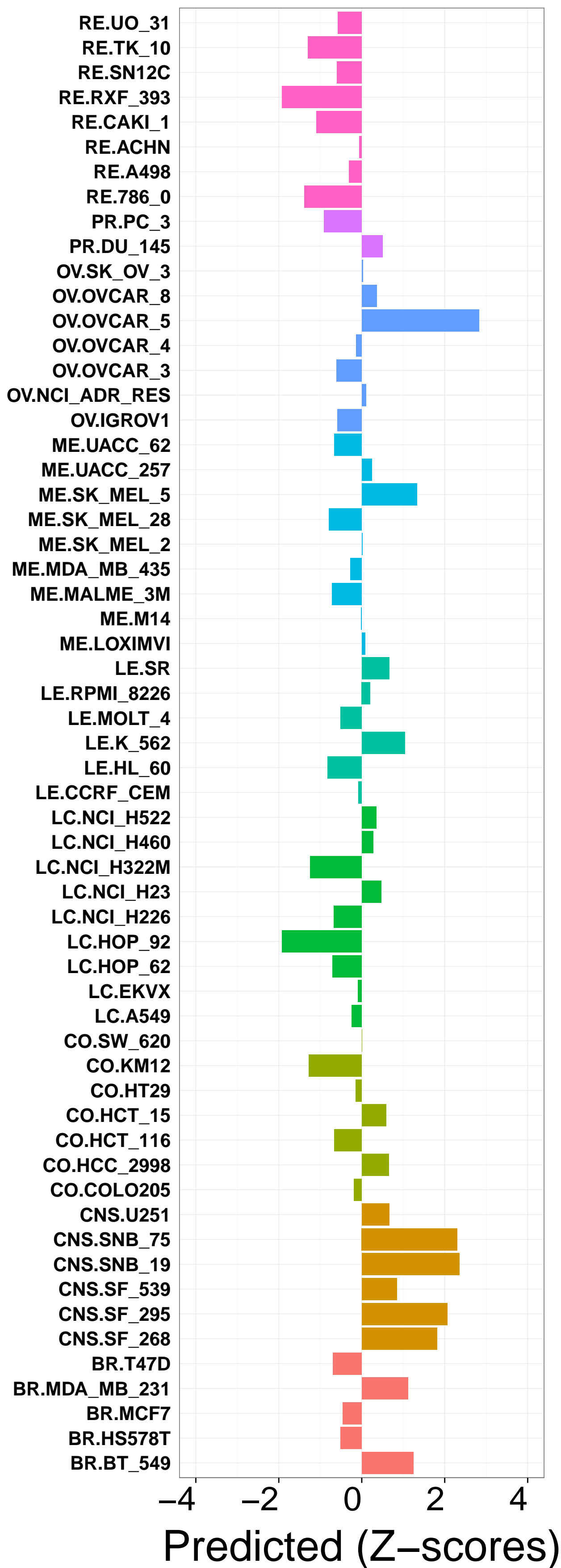
Observed (Z-scores)
