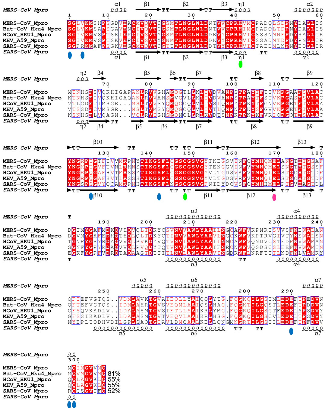
S1 Fig. Sequence alignment of betacoronaviral M pro .
